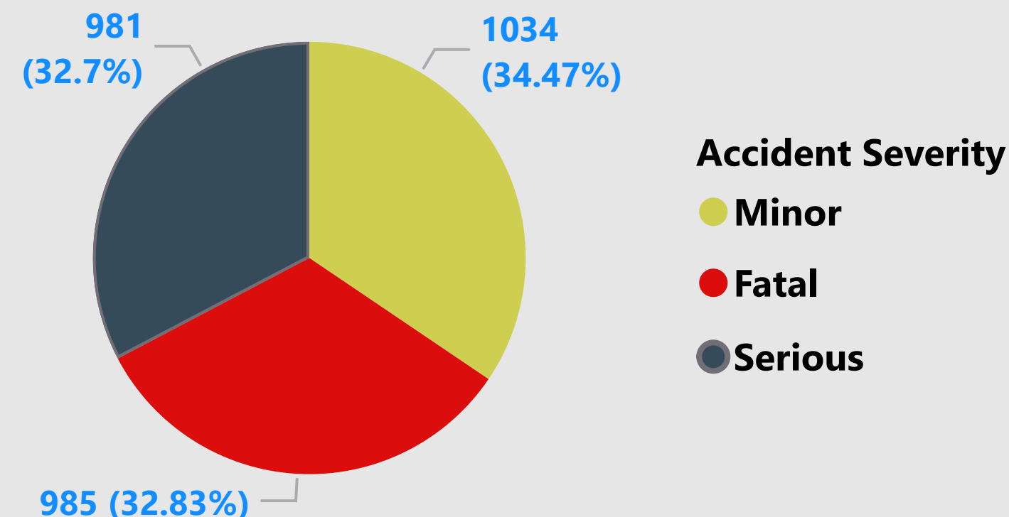
Accident Severity
