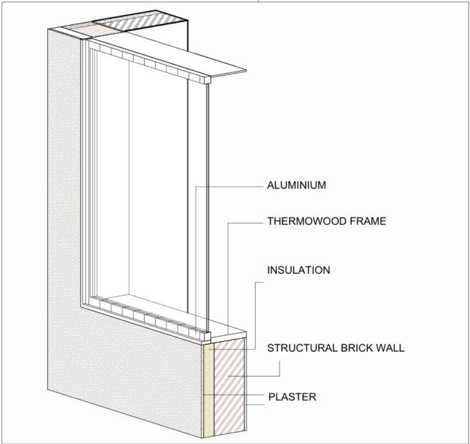
WINDOW DETAIL STRATIGRAPHY
