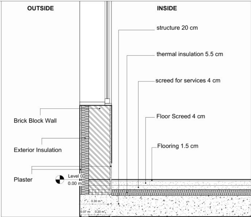
GROUND FLOOR DETAIL EXTERNAL WALL SECTION
