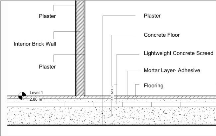
FIRST FLOOR DETAIL INTERNAL WALL SECTION DETAIL
