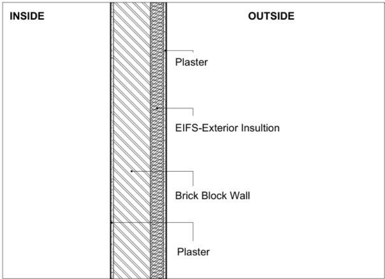
EXTERNAL WALL SECTION
