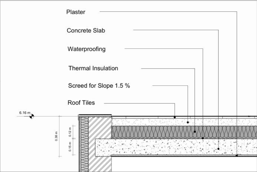
ROOF DETAIL STRATIGRAPHY
