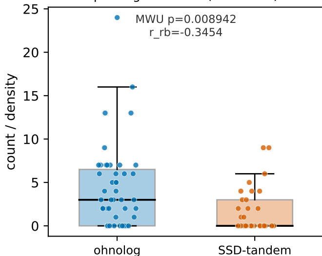
CTCF peaks between paralog members (raw count)
