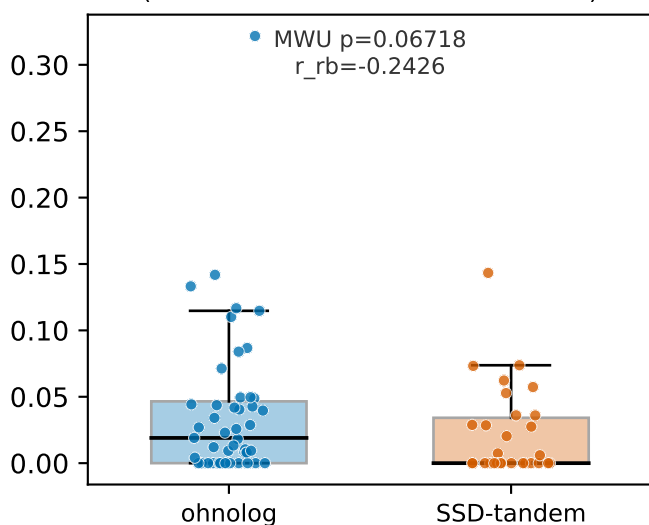
CTCF peaks/kb between members (inter-member-distance normalized)
