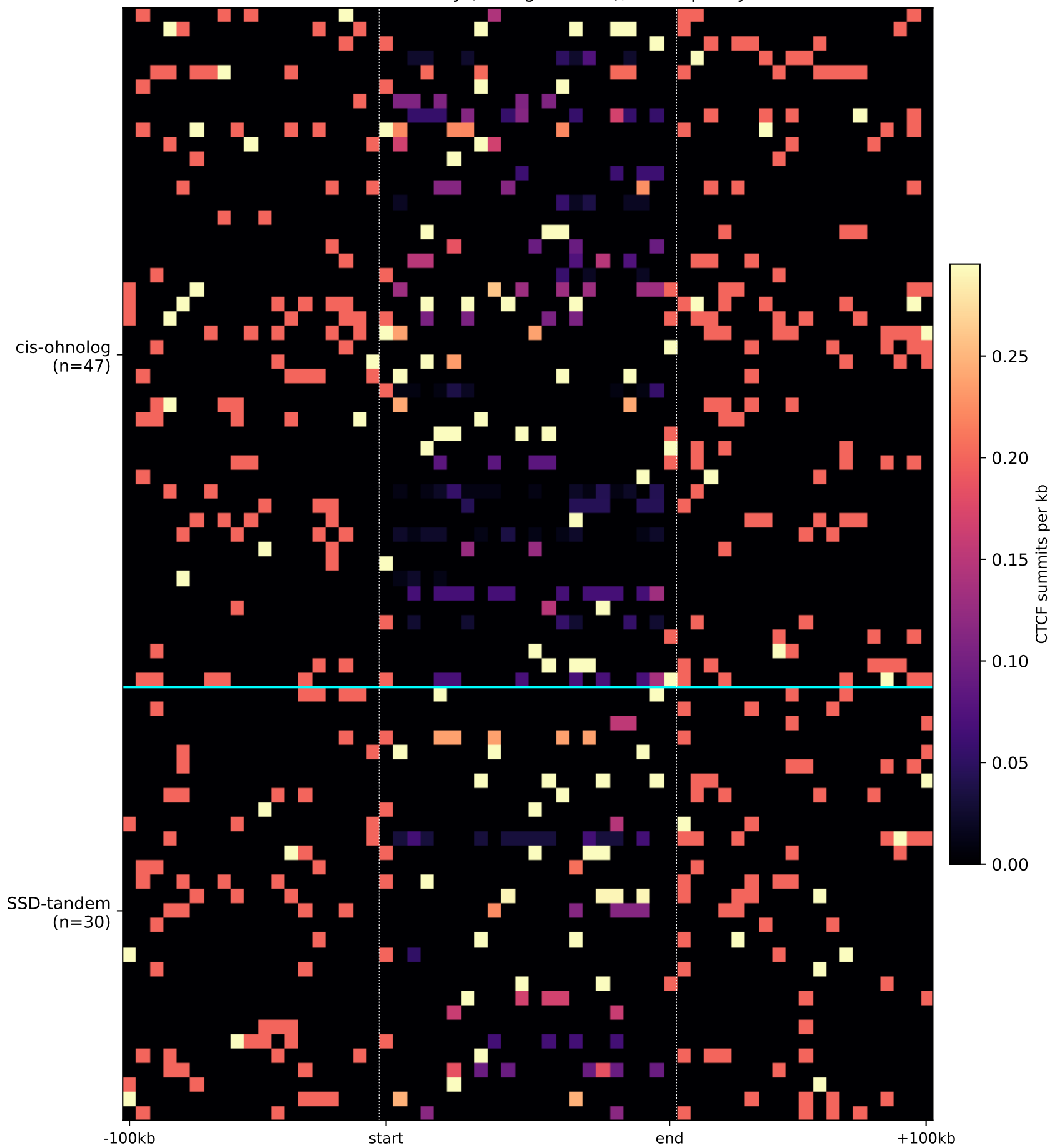
Per-locus CTCF density (metagene bins), rows split by class
