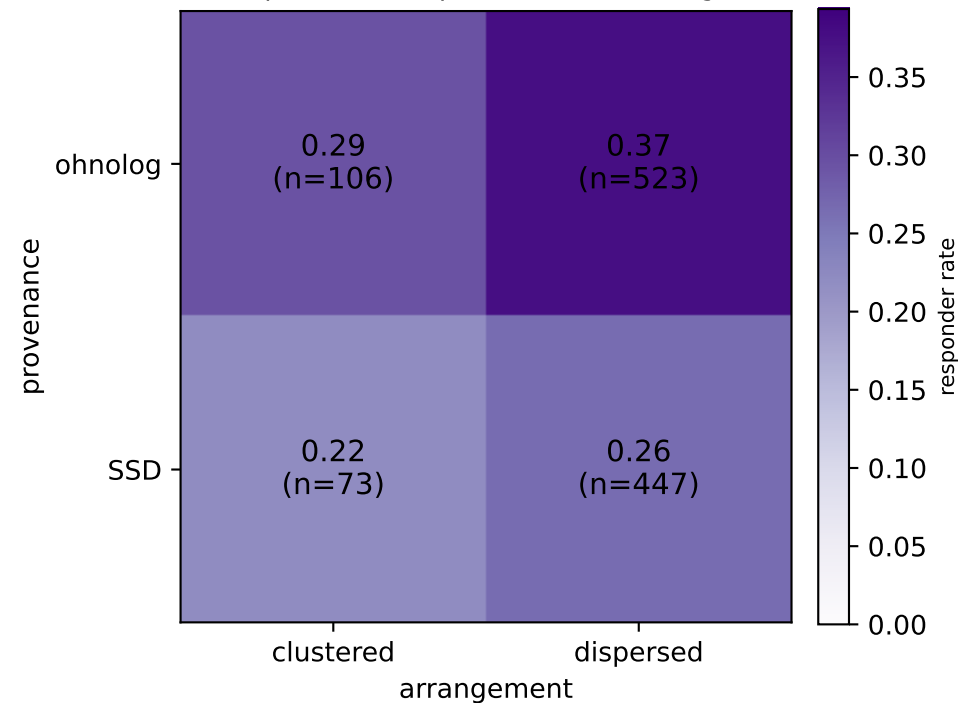
(B) Responder rate: provenance x arrangement
