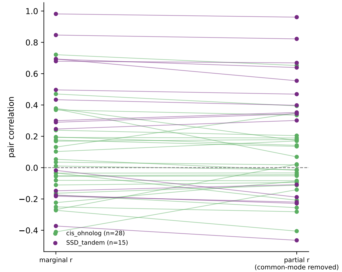
(C) Neighbor pairs: shared-drive vs compensation
