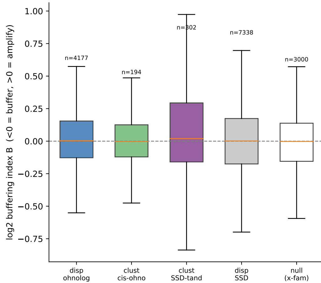
(A) Buffering index by category
