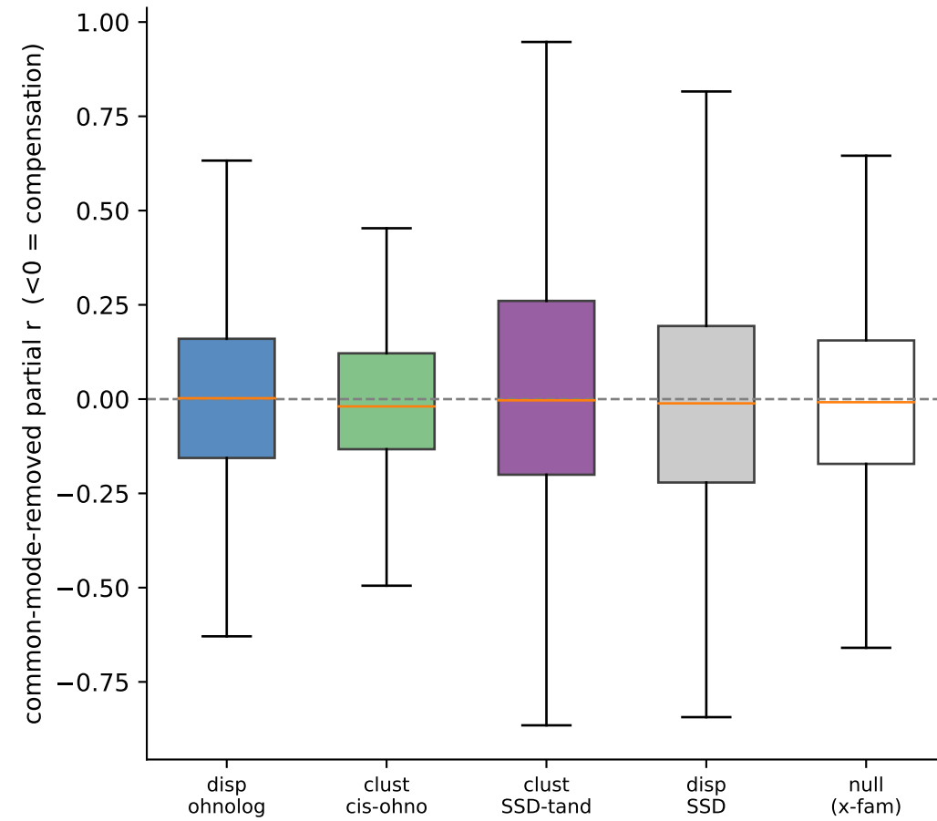
(B) Compensation (partial r) by category
