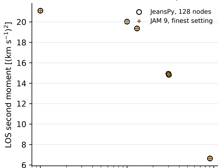
Plummer tracer: intrinsic q = 1
