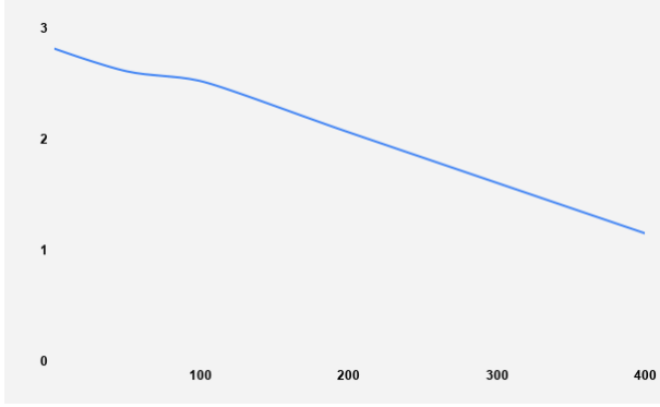
Figure 4: Diagram showing the relation of chsh and distance
