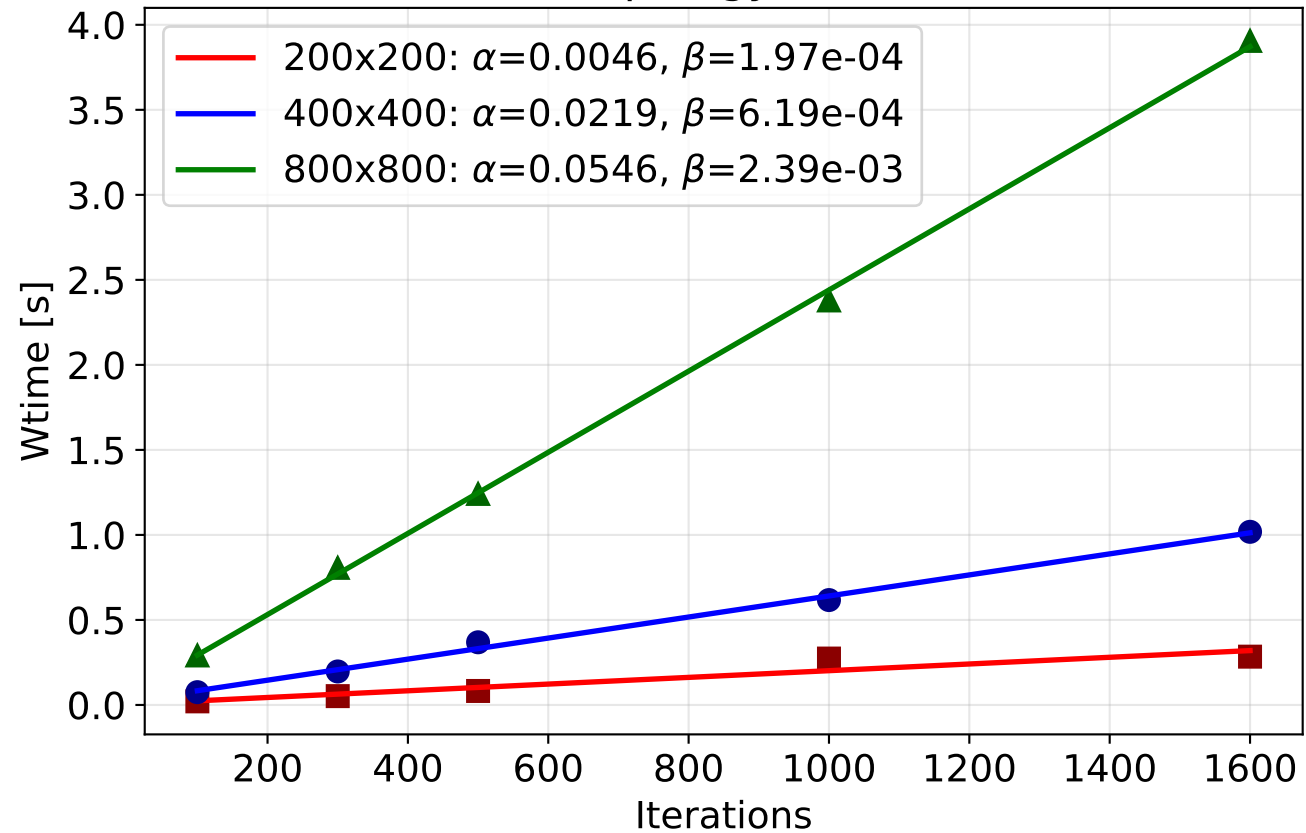
Topology 4x1
