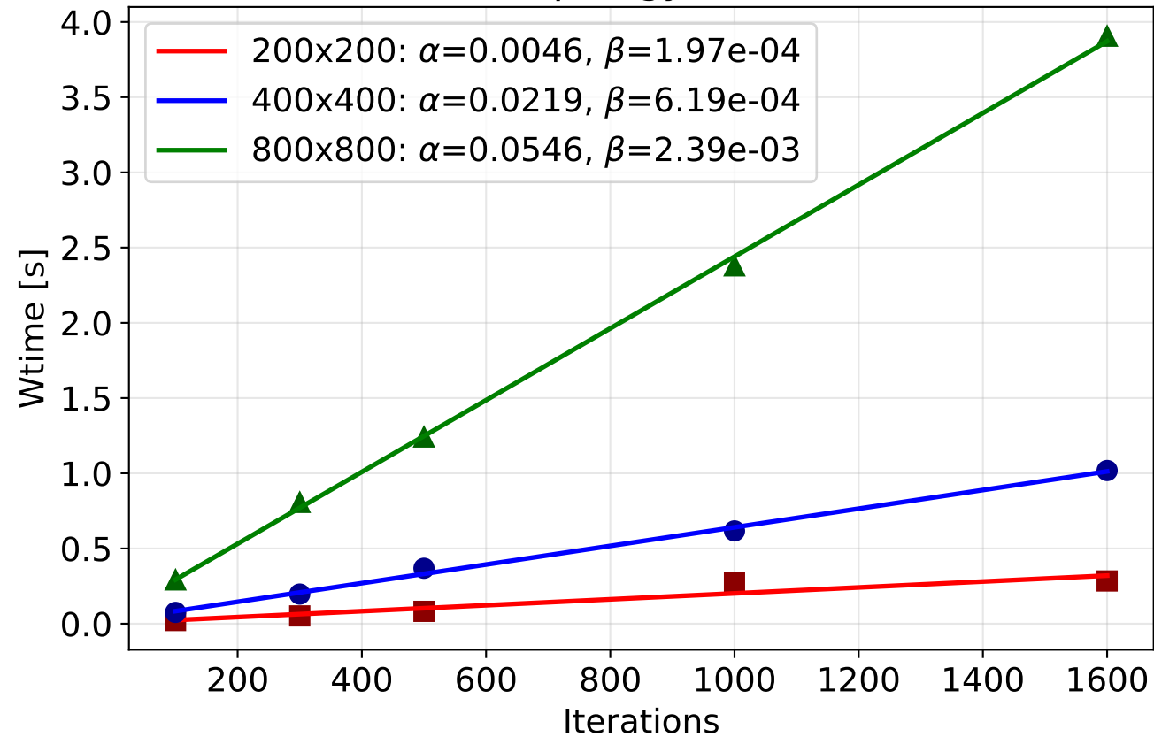
Topology 4x1
