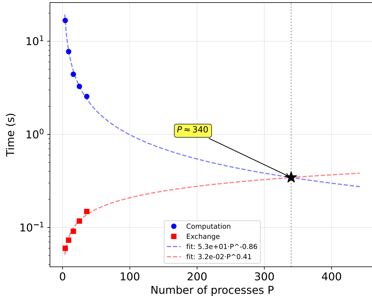
N=1000, block
