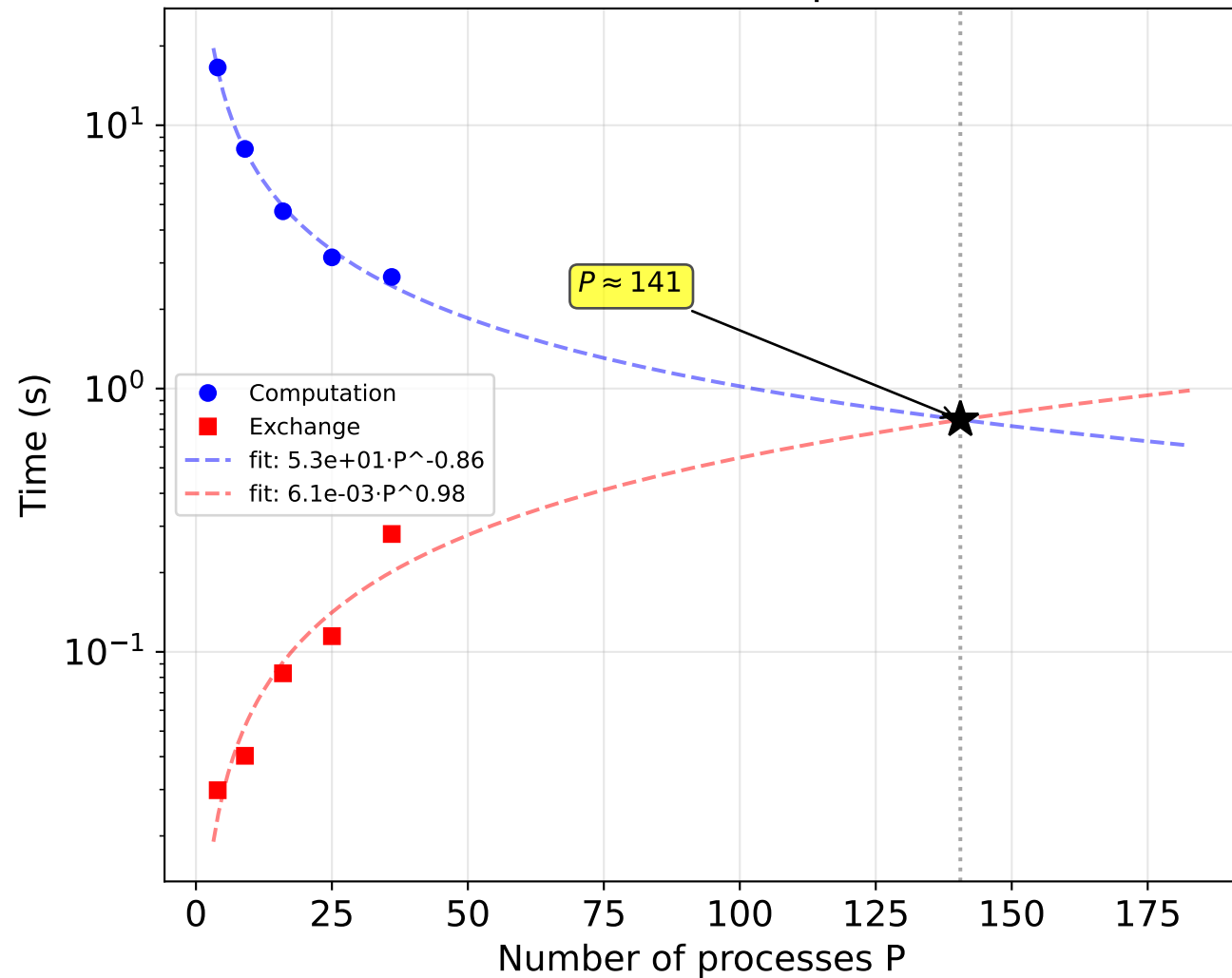
N=1000, stripe
