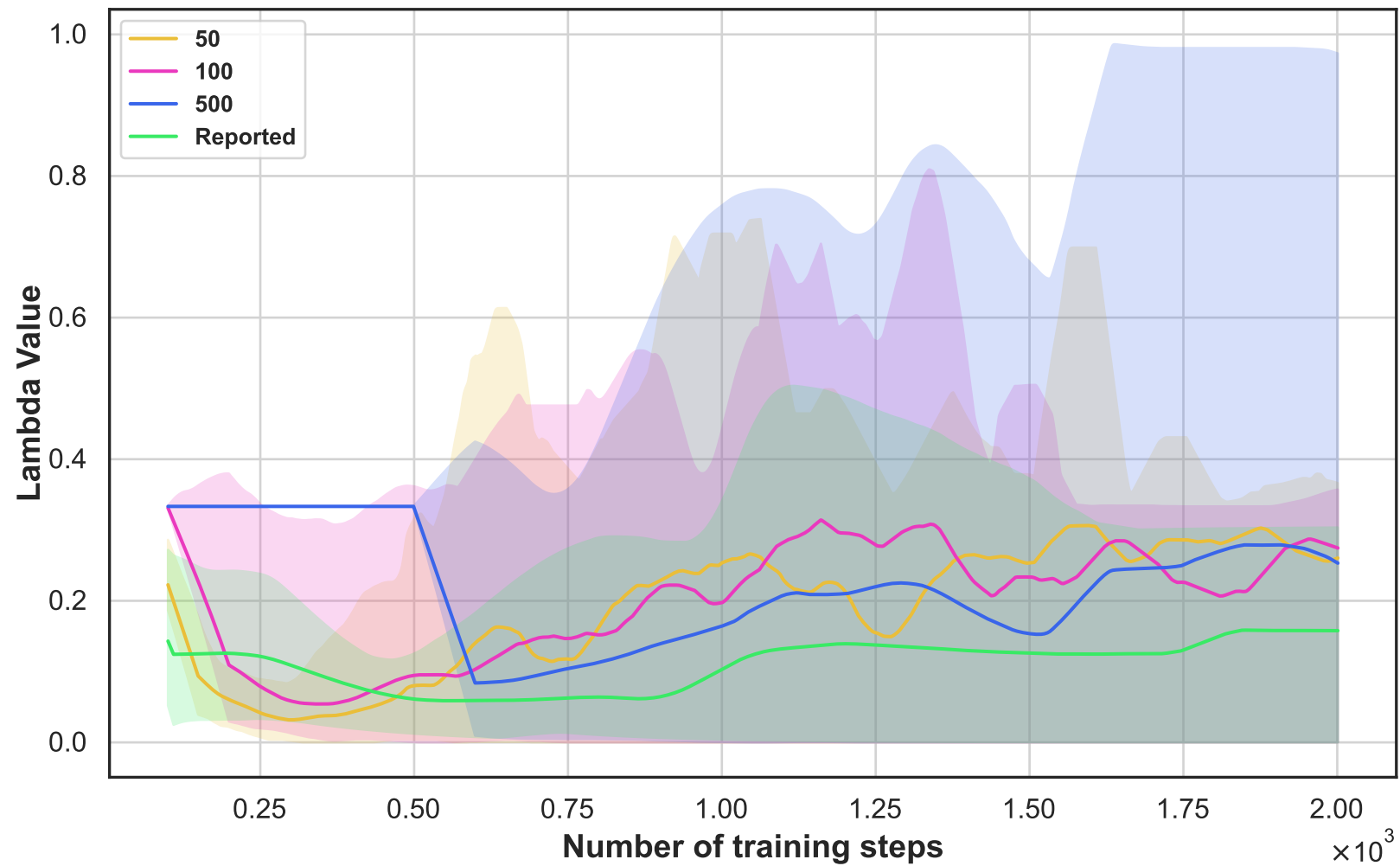
Banana Lambda - Different RB Values
