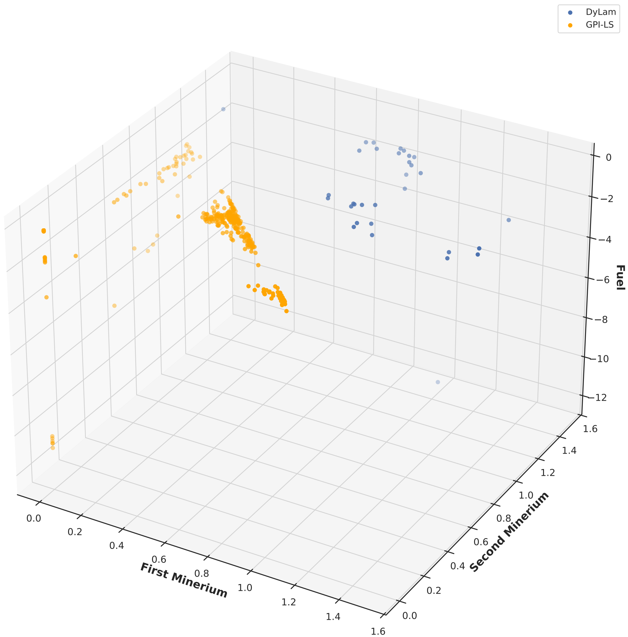
Pareto frontier comparison - Minecart
