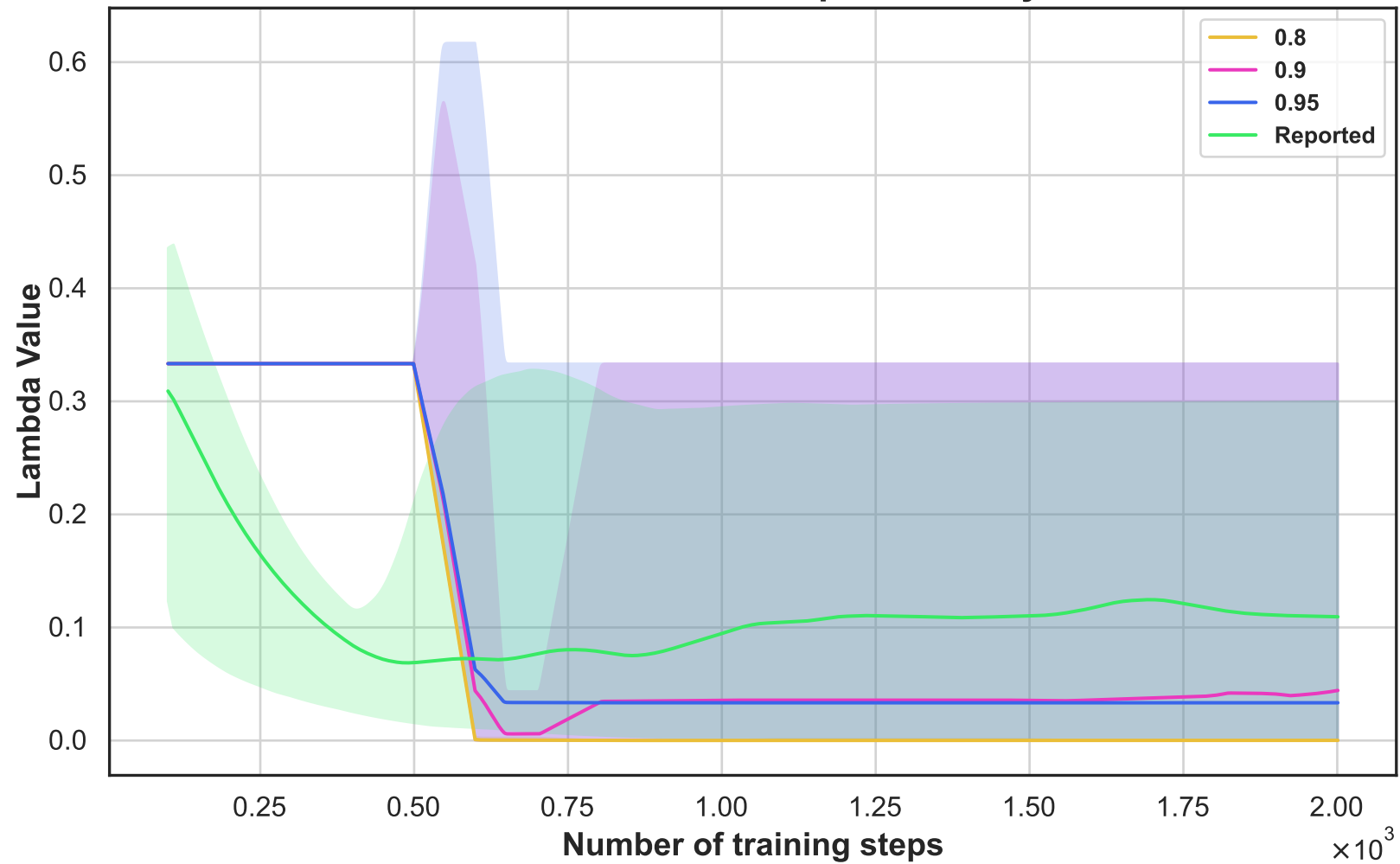
Gate Lambda - Different Epsilon decay rates
