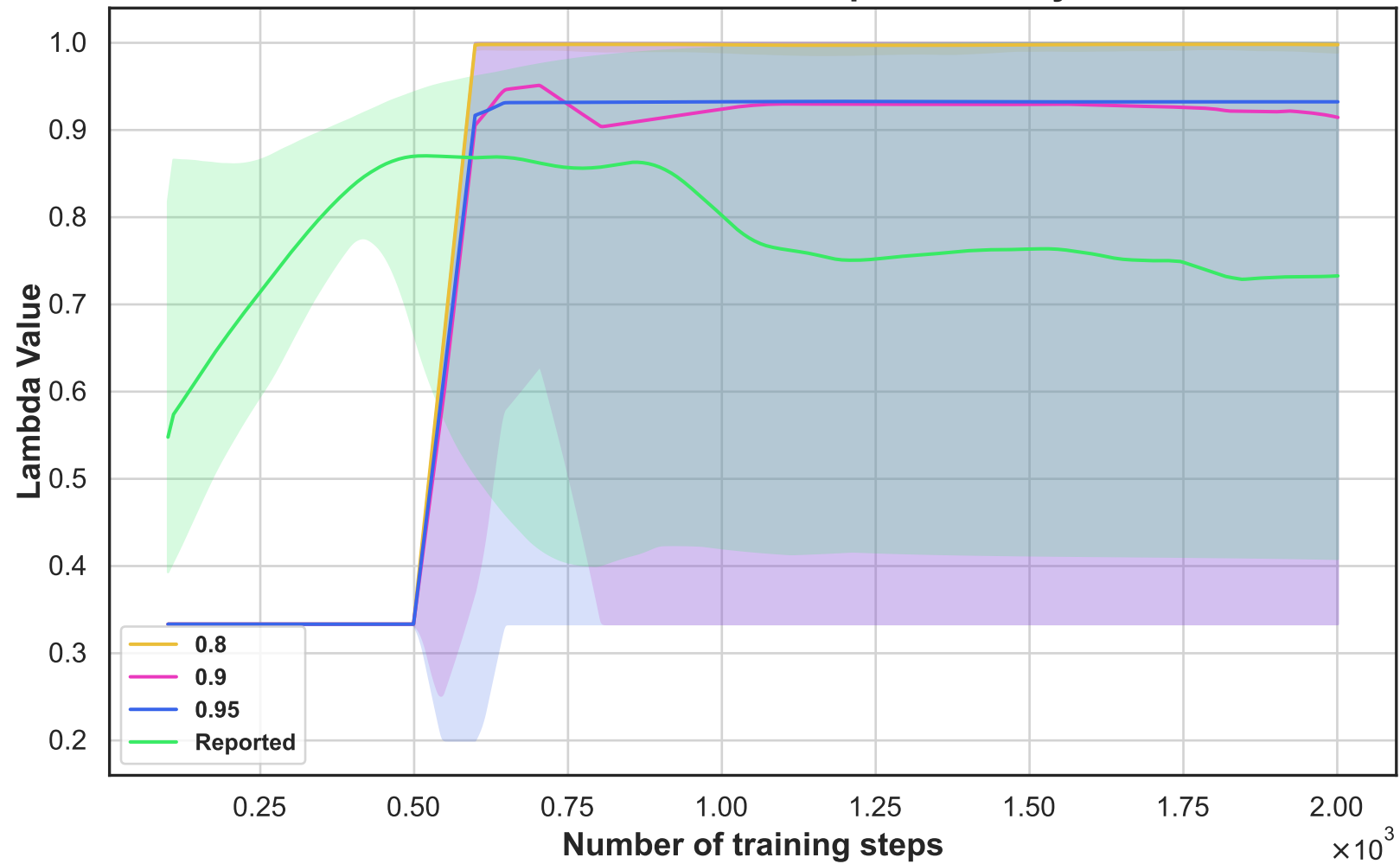
Chicken Lambda - Different Epsilon decay rates
