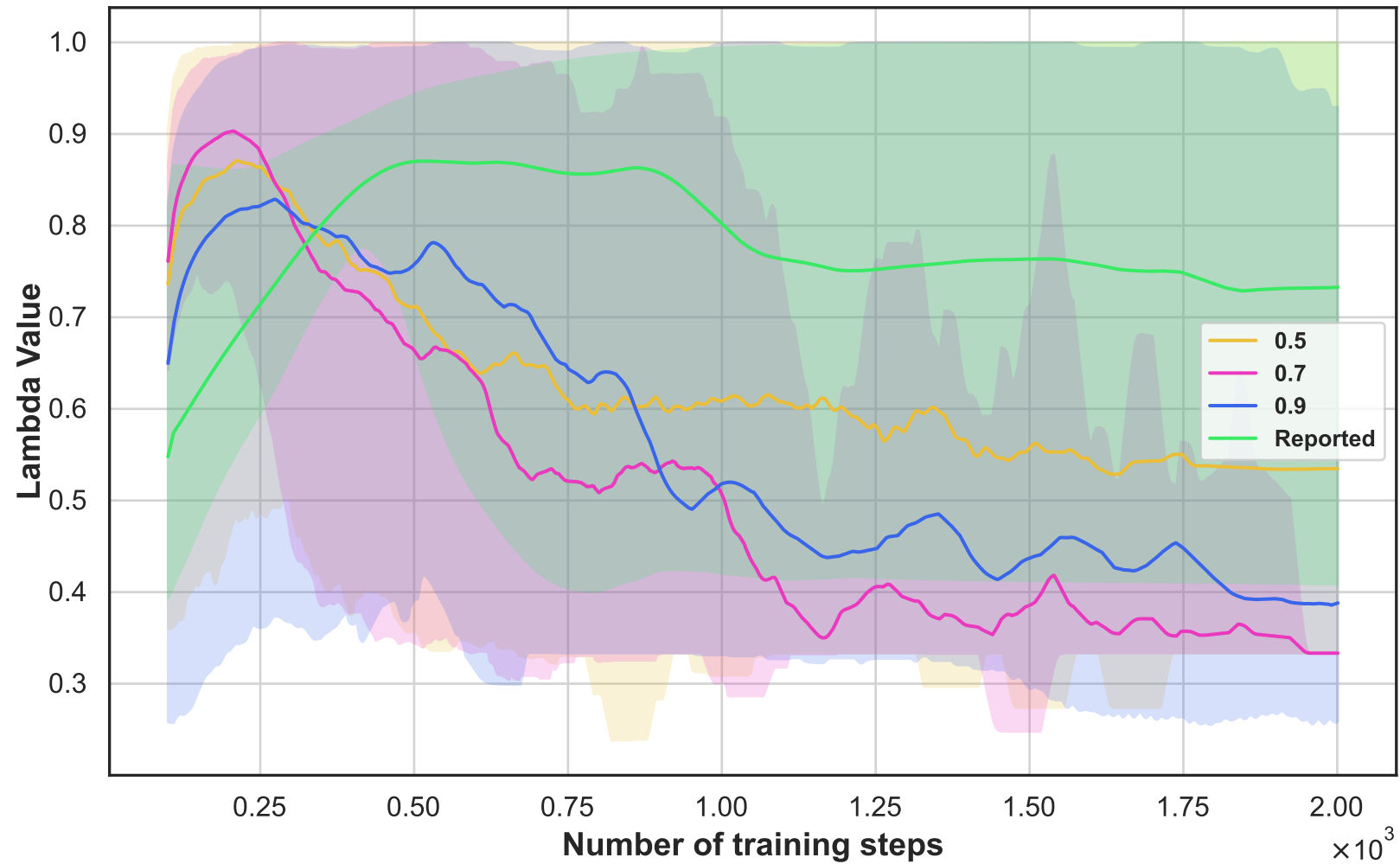
Chicken Lambda - Different Tau Values
