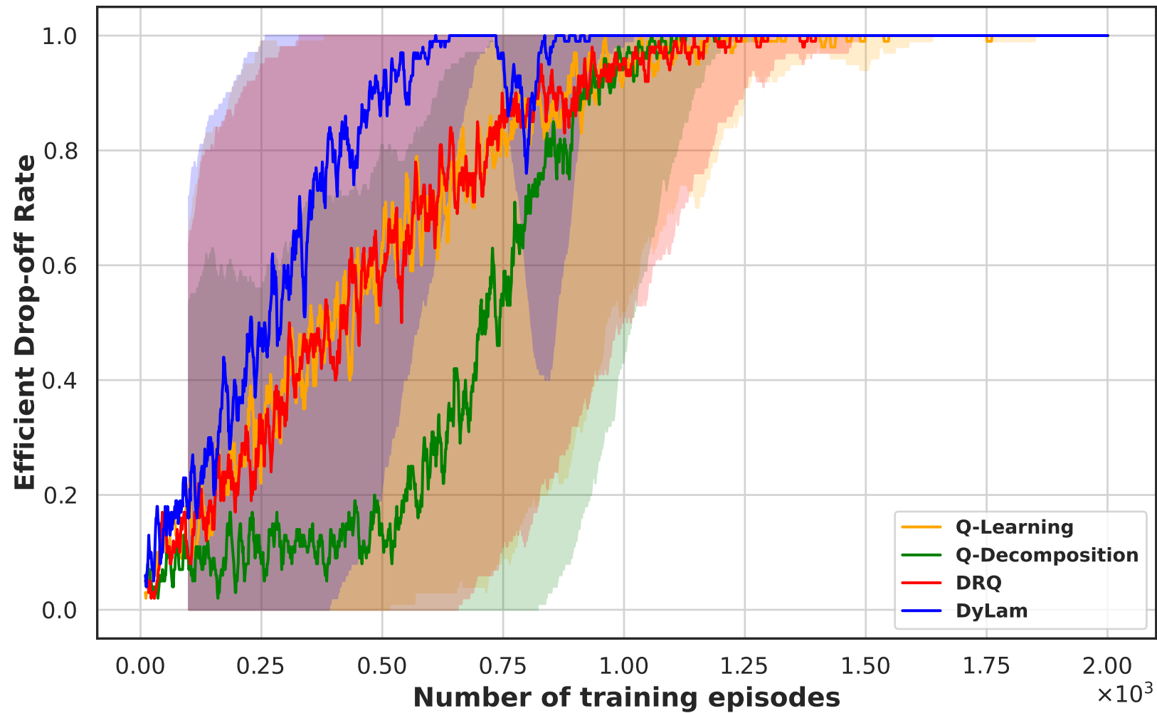
Taxi-v3
