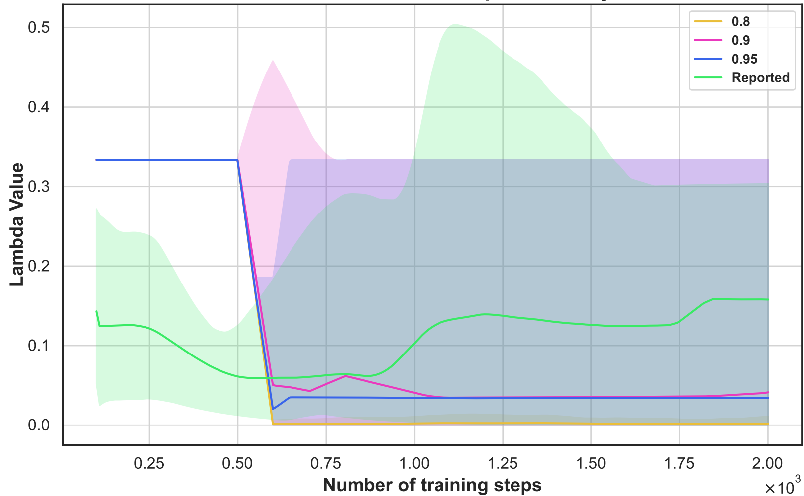
Banana Lambda - Different Epsilon decay rates
