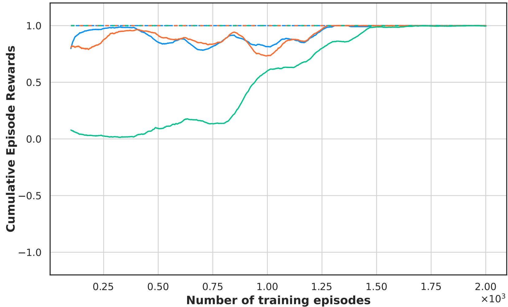
ChickenBanana-v0
