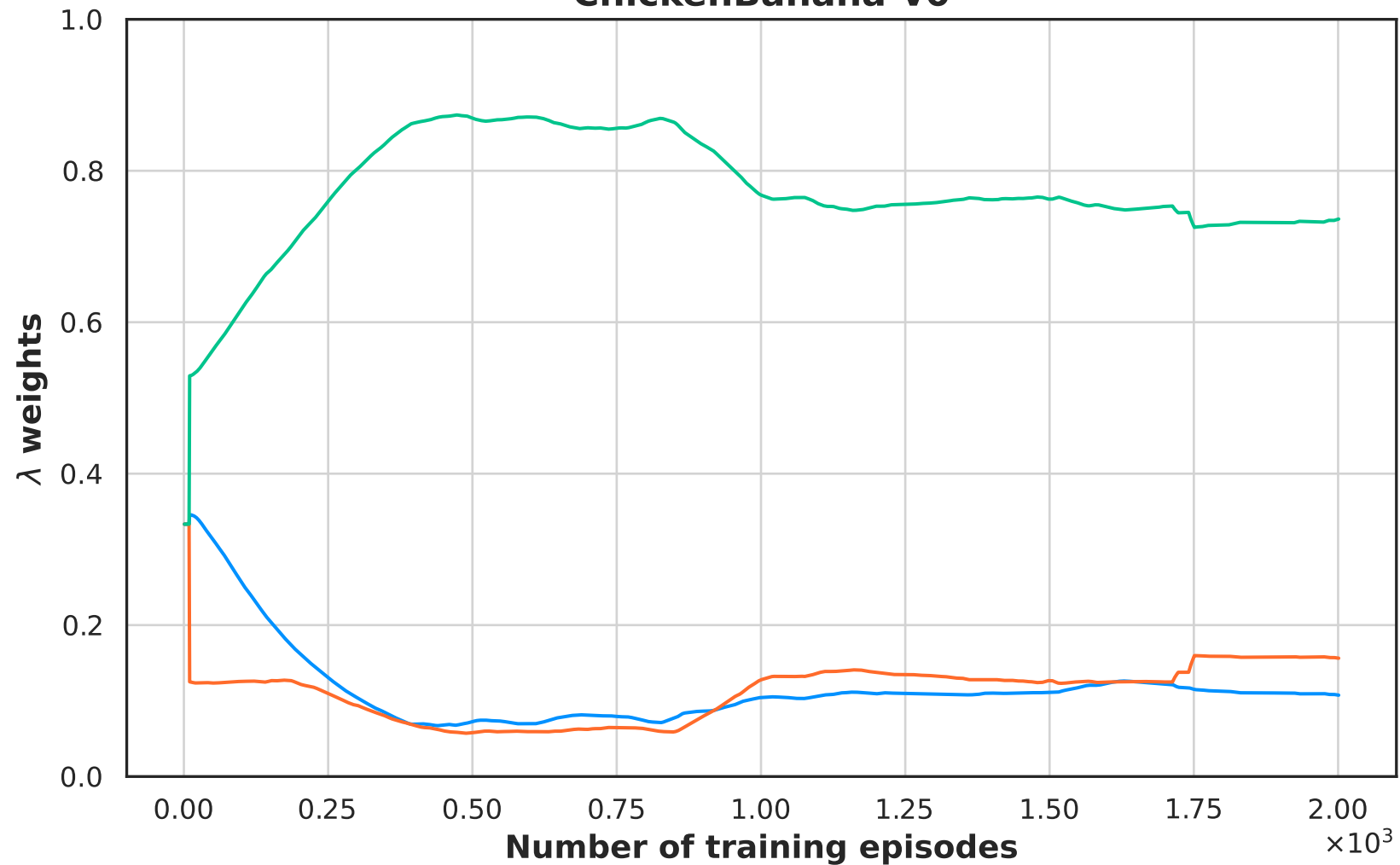
ChickenBanana-v0
