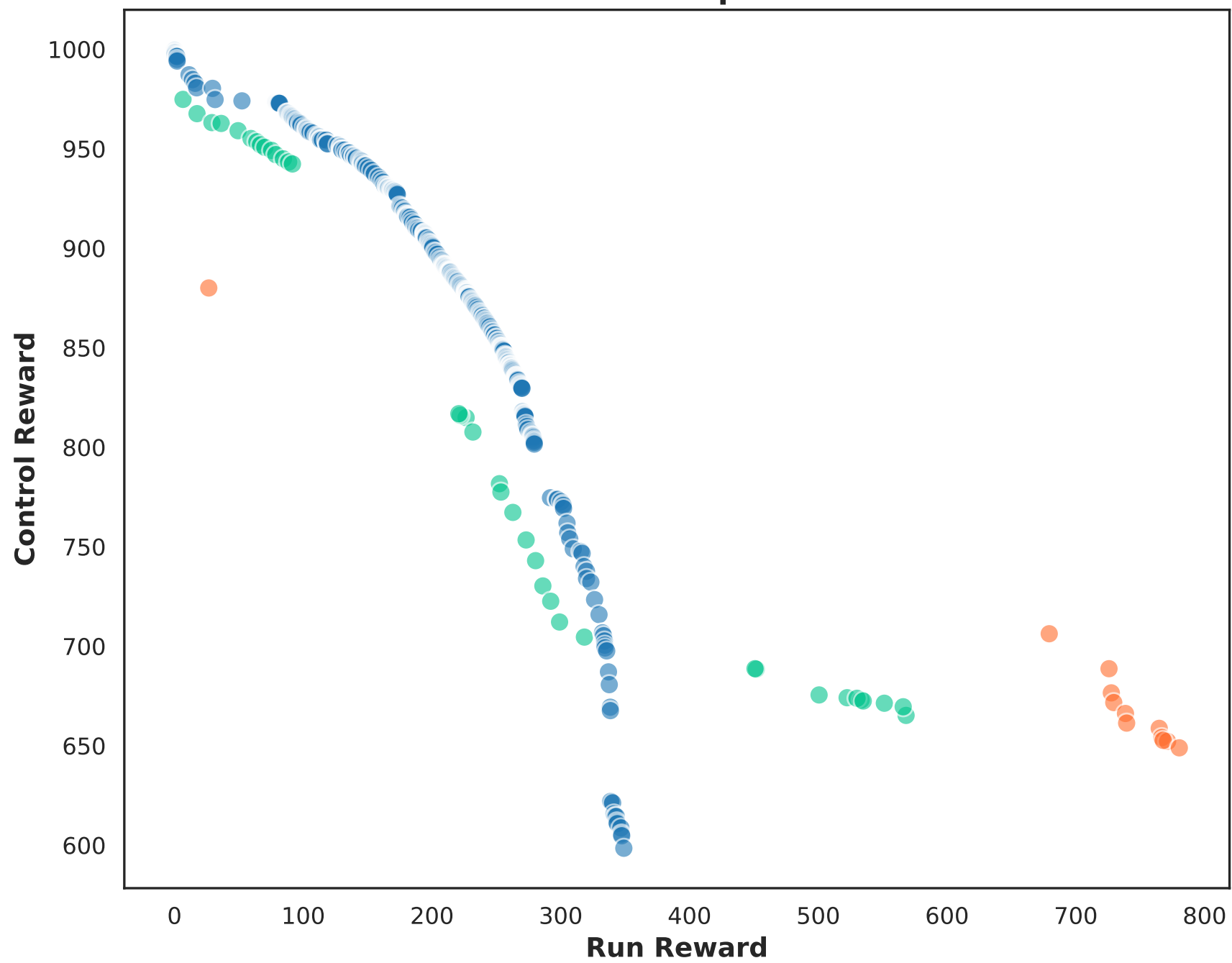
Reward Space
