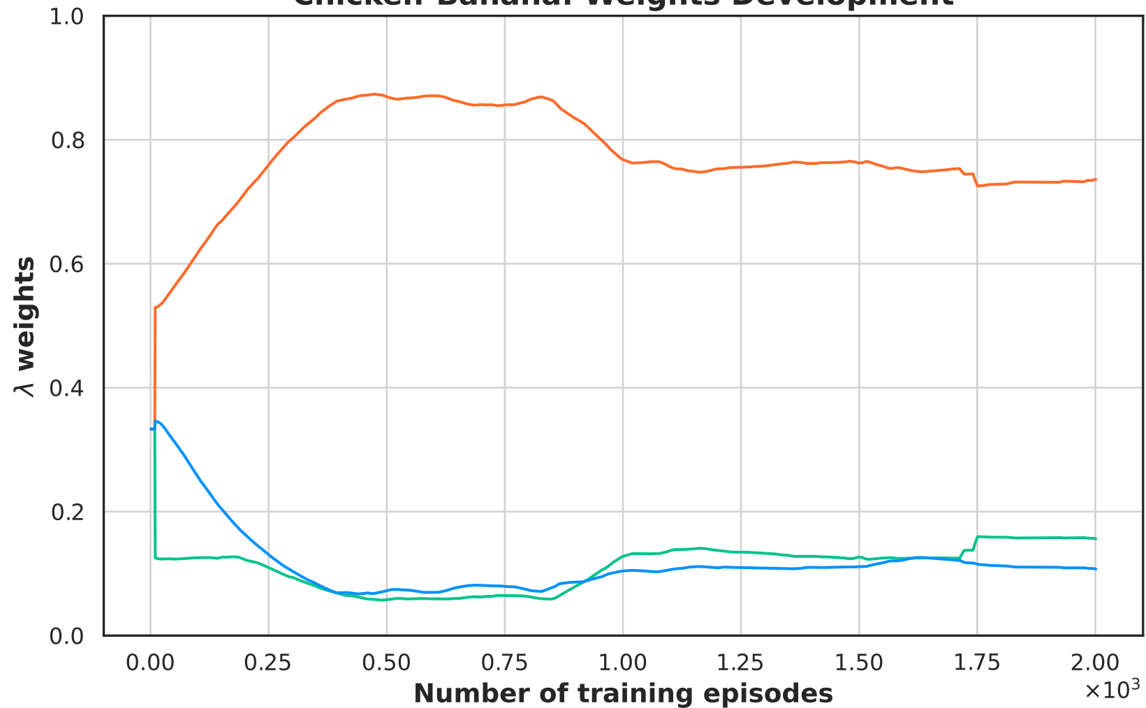
Chicken-Banana: Weights Development
