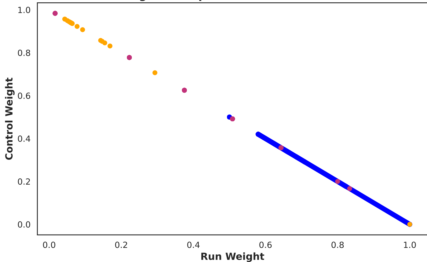
Weights Comparison for HalfCheetah
