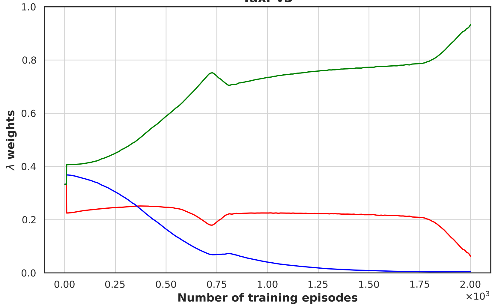
Taxi-v3
