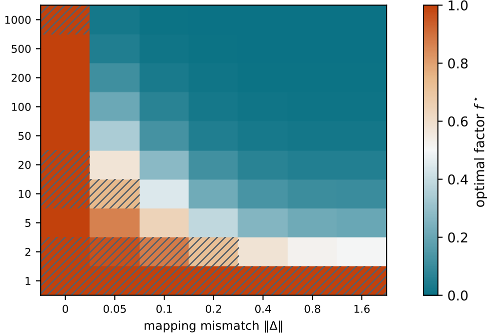
Closed form \min \{1, (1 + c)/(a + c)\}
