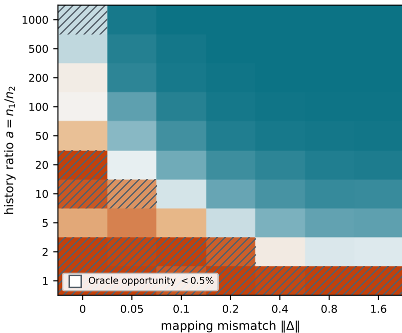
Conditional Oracle f^* (population risk)
