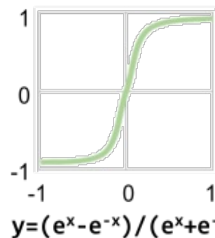
Hyperbolic Tangent
