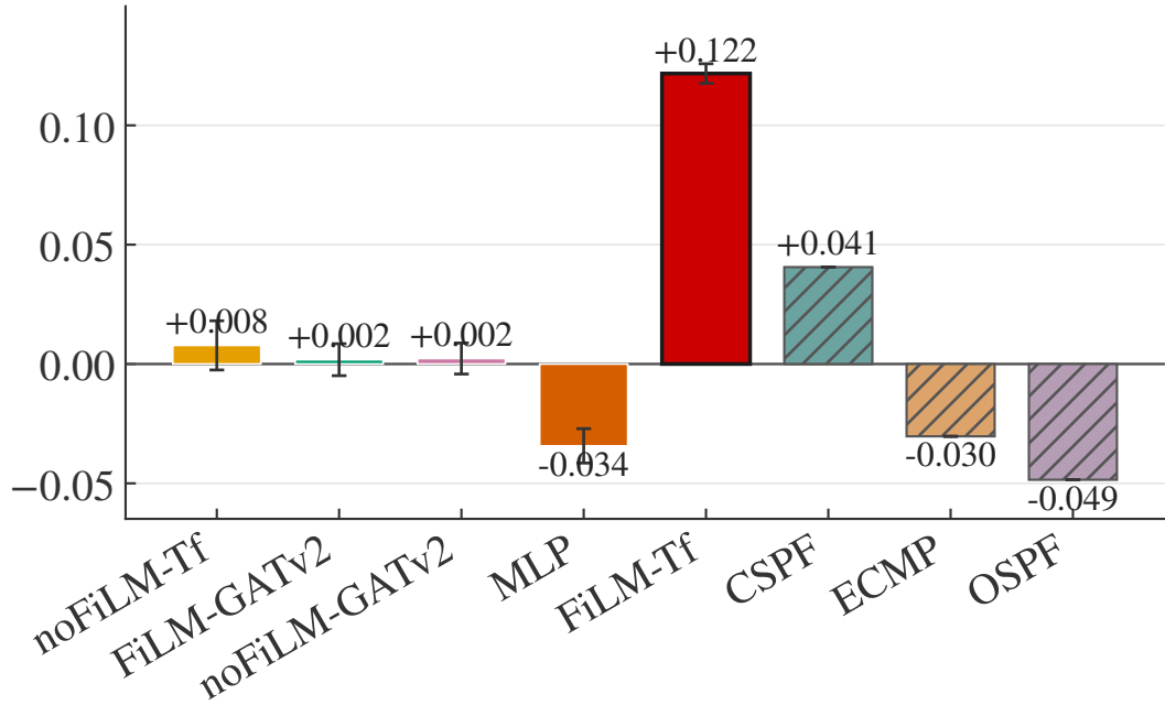
Mean Reward
