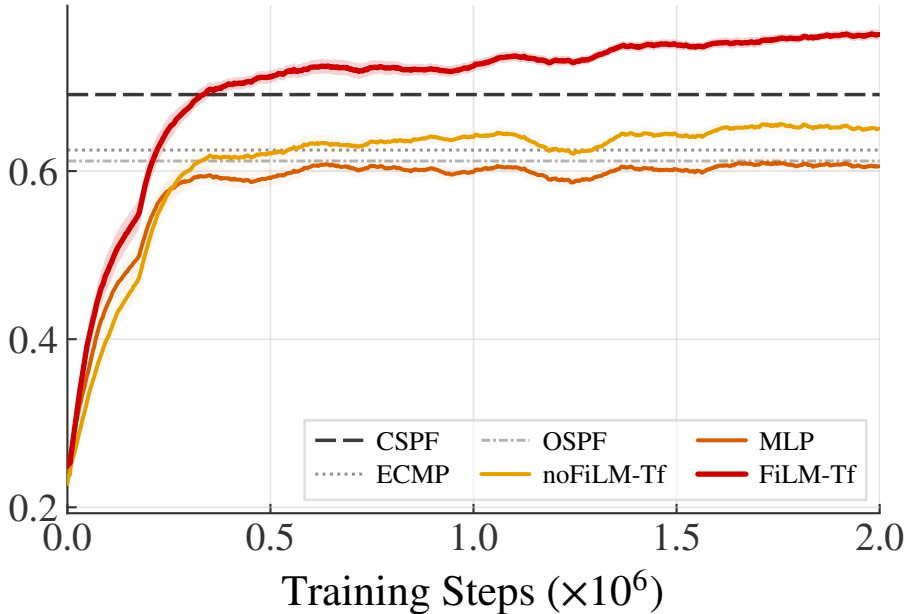
Bandwidth Score
