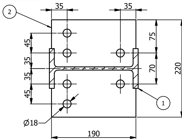
CUT D-D
