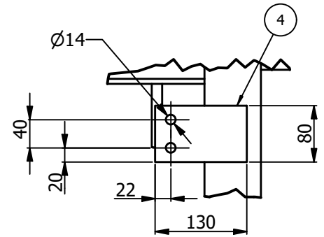
DETAIL ESCALA:(1: 7.5)
