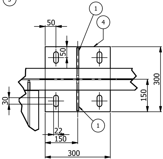
DETAIL D
