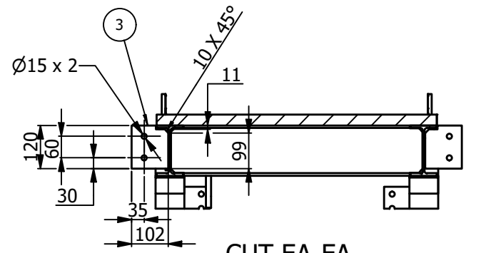
CUT EA-EA ESCALA:(1 :15)
