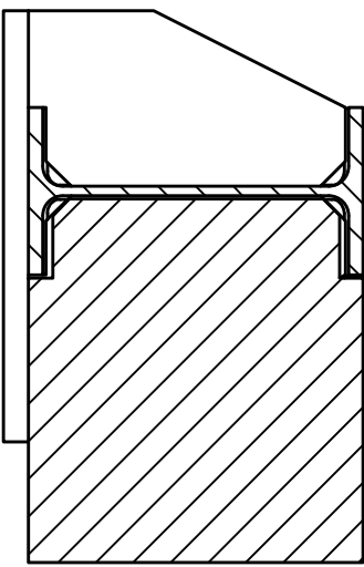
CUT B-B
