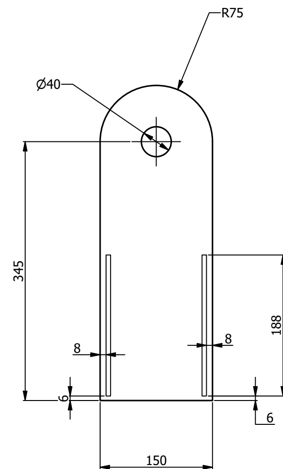
FRONT VIEW ESCALA:(1 : 5)
