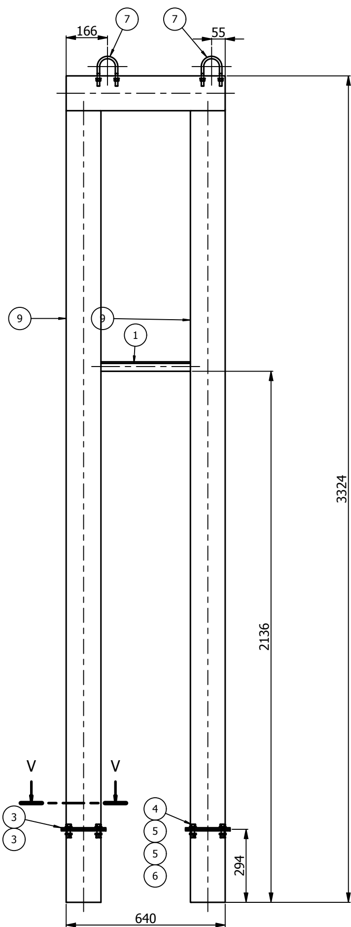
VISTA FRONTAL
