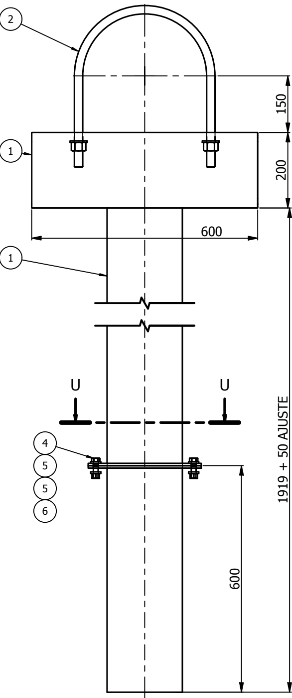
VISTA FRONTAL
