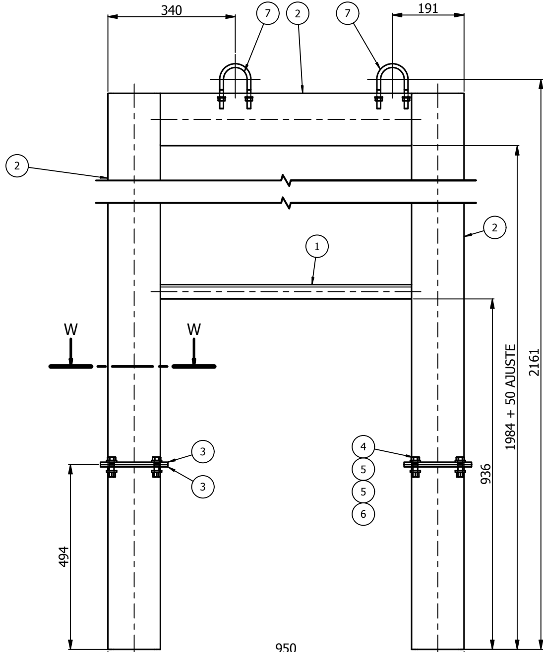
VISTA FRONTAL
