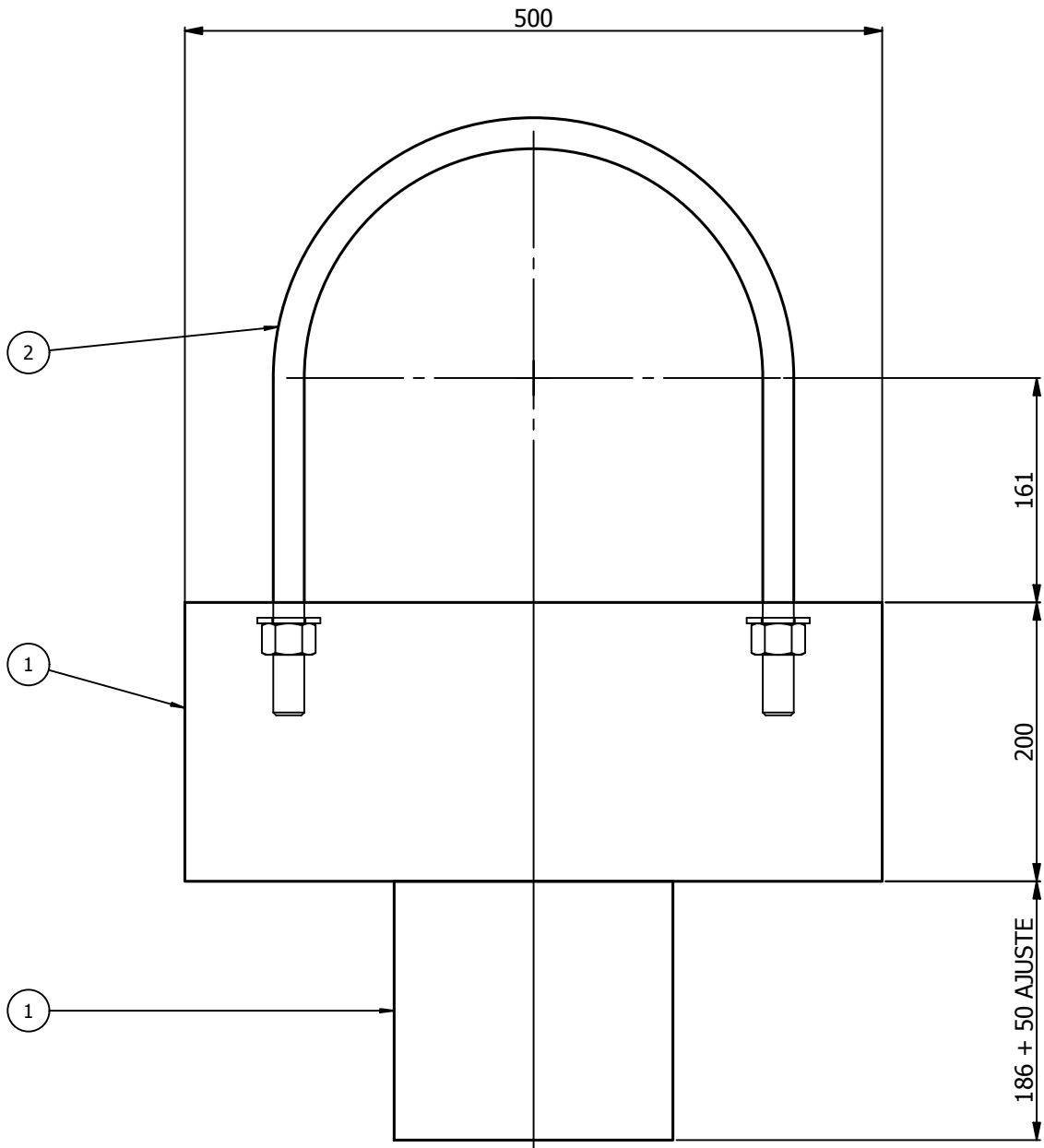
VISTA FRONTAL
