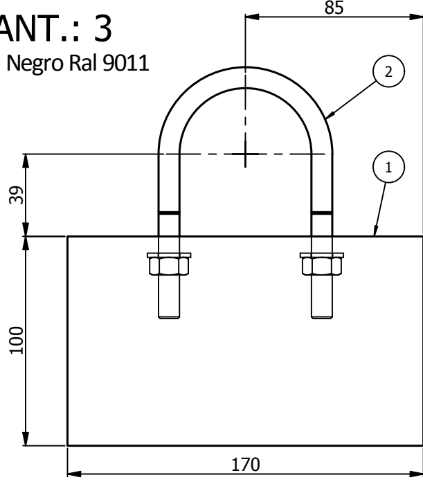
VISTA FRONTAL
