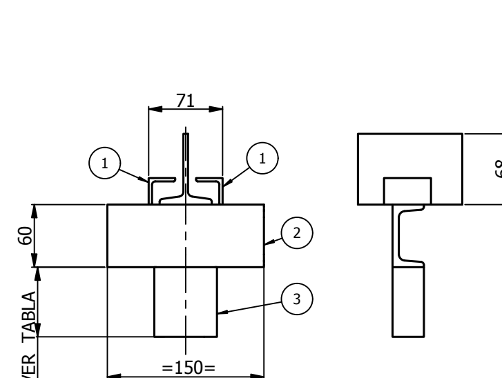
VISTA FRONTAL
