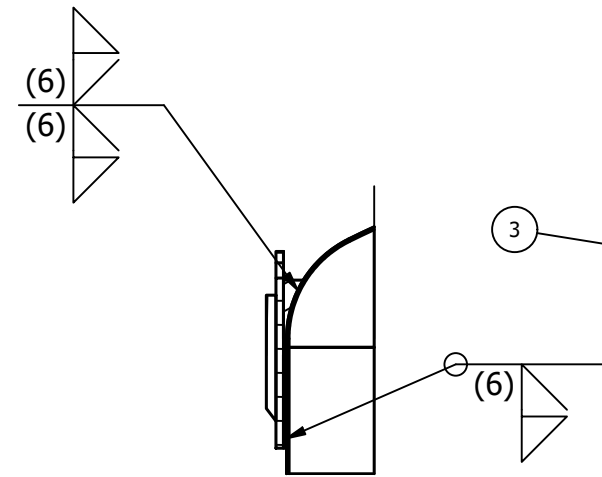
CUT DN-DN
