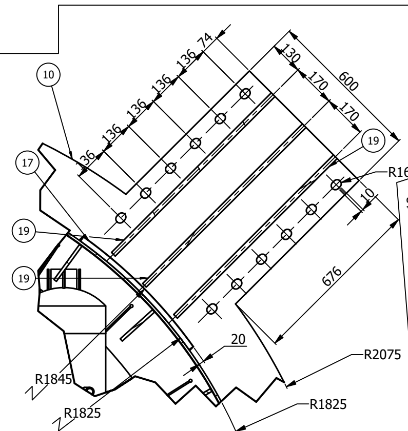
DETAIL C
