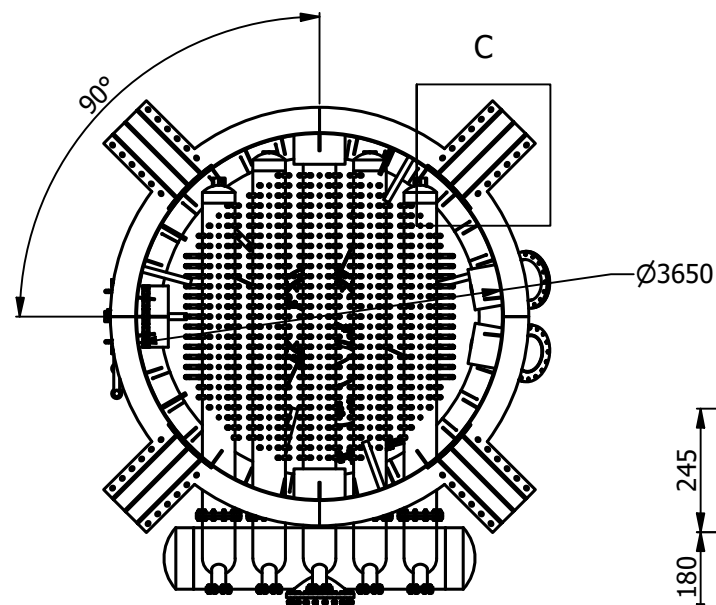
EQUIPMENT SUPPORT LEGS VIEW
