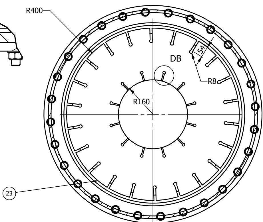
CUT DA-DA NOTE: THIS PIECE IS SIMPLY SUPPORTED, DO NOT WELD ESCALA:(1 : 10)
