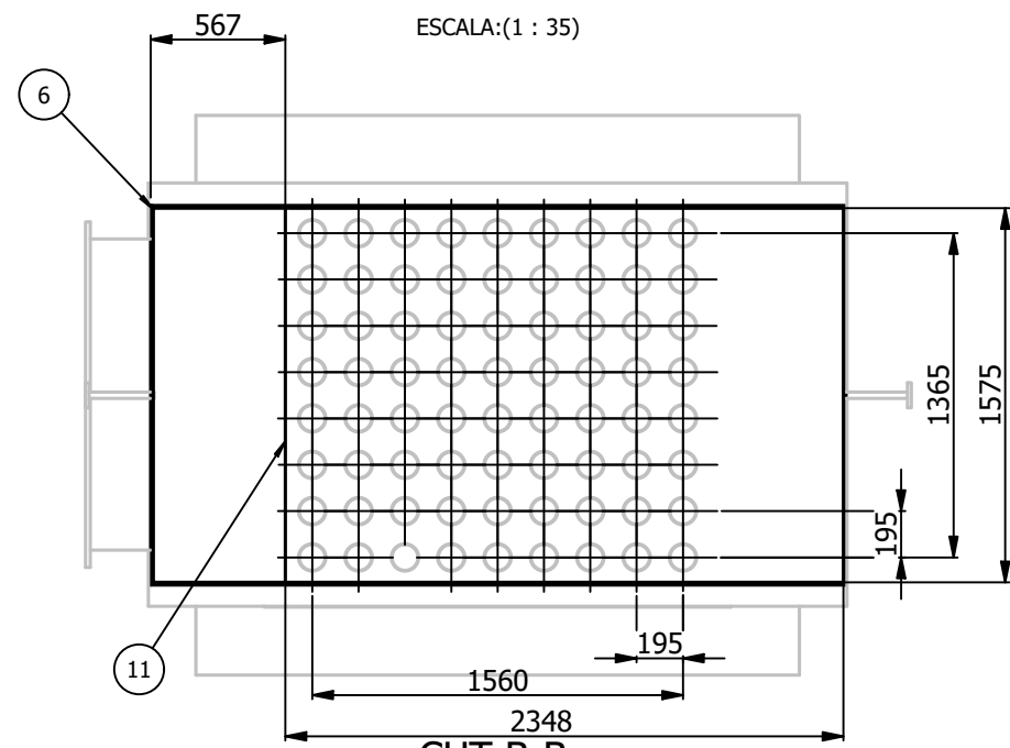
CUT B-B
