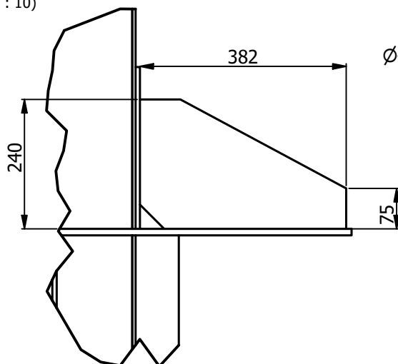
DETAIL BY ESCALA:(1 : 10)
