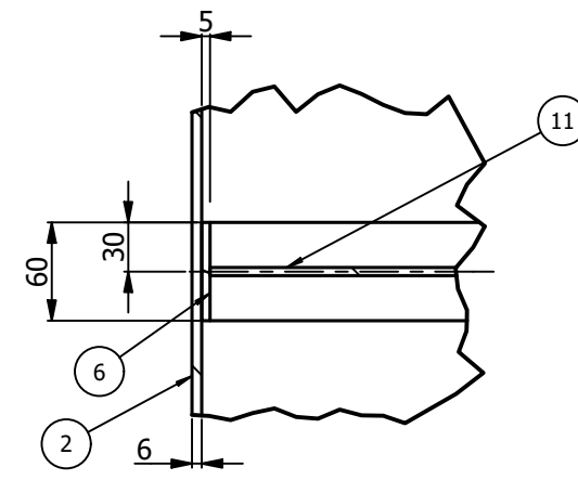
DETAIL F
