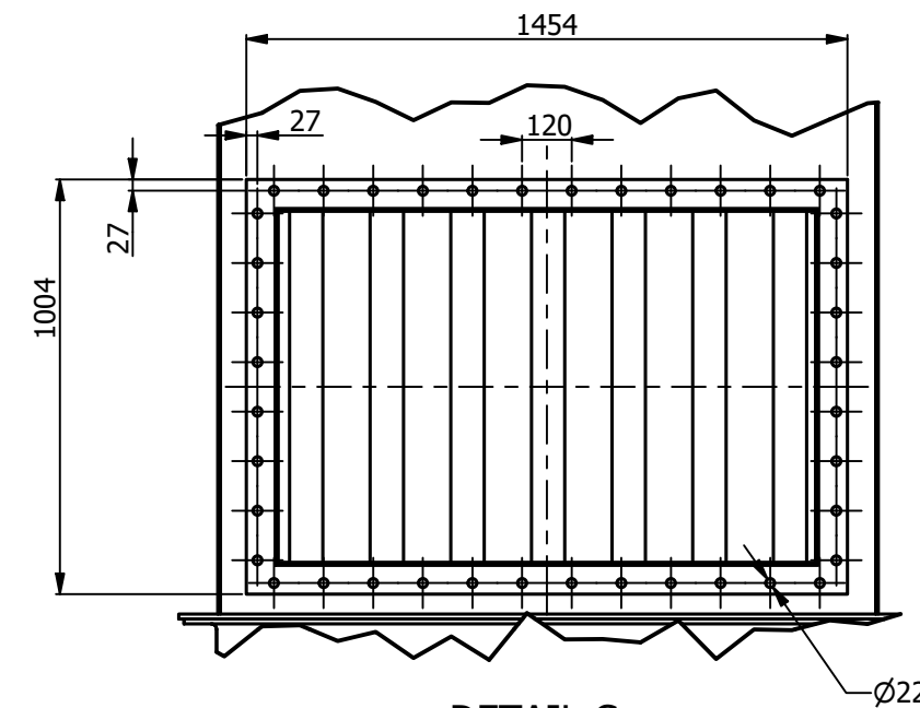
DETAIL C
