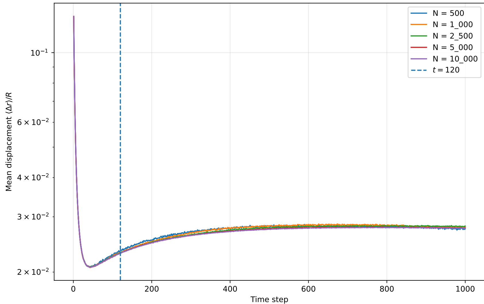
Initial mechanical relaxation, \rho = 0.85
