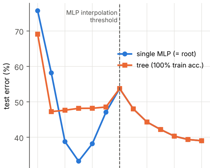
CIFAR-10, n=4000, 20% label noise
