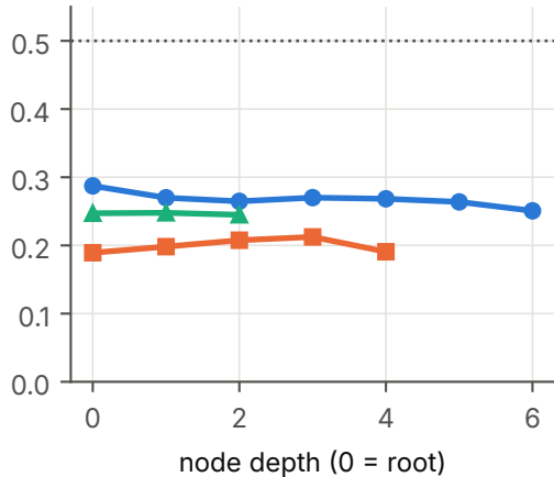
Cats vs Dogs: area holding 50% of saliency
