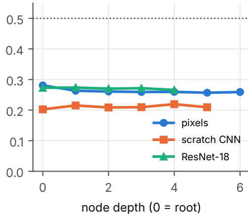
CIFAR-10: area holding 50% of saliency
