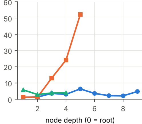
CIFAR-10: positives fired by bias alone (%)
