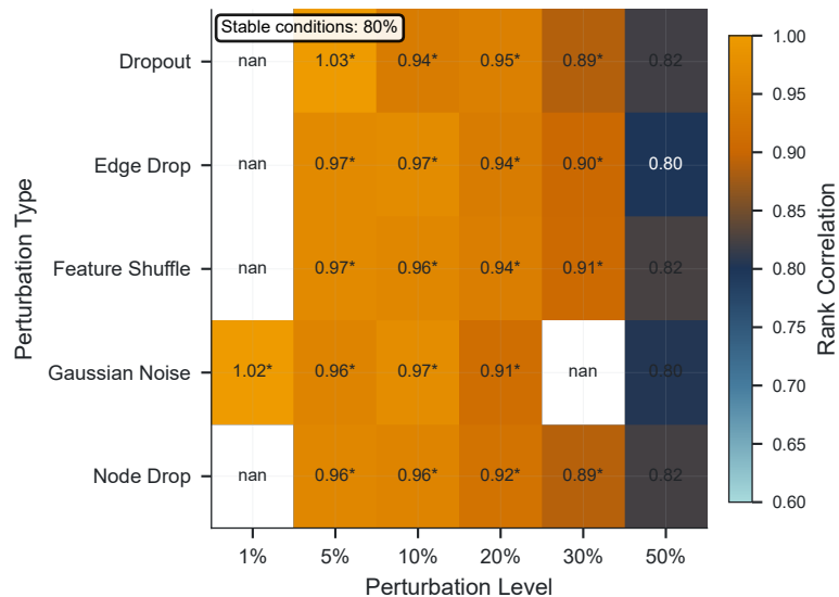
b Perturbation Robustness Analysis
