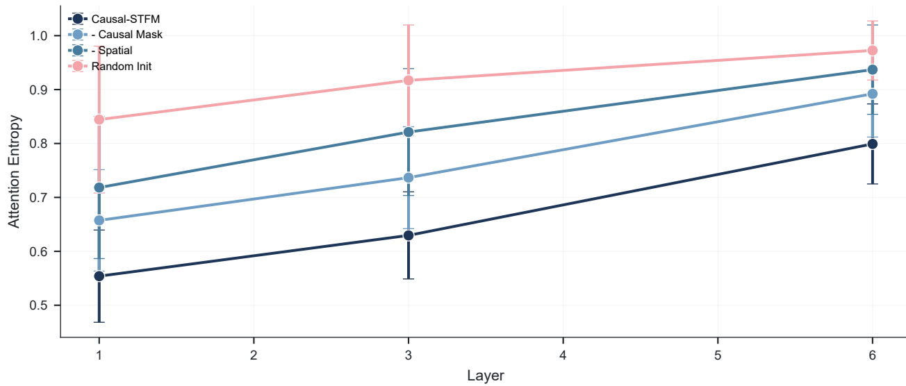
Entropy Across Layers
