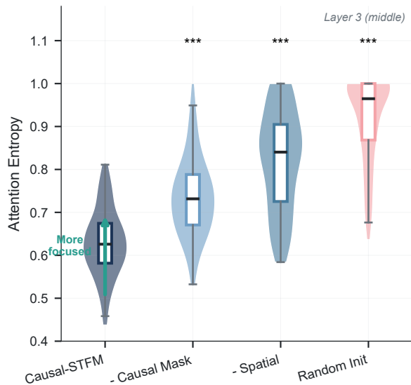
a Attention Entropy by Model Variant
