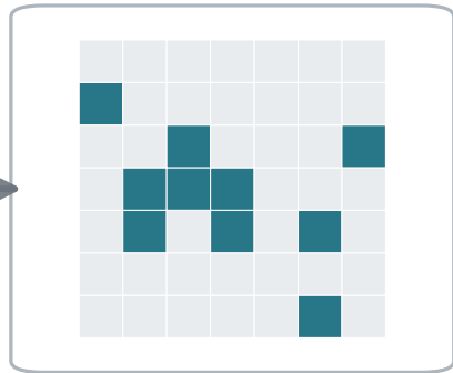
Masked Attention
