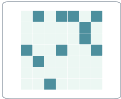
Attention Matrix
