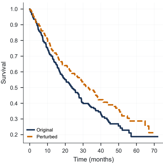
PD1-PDL1
