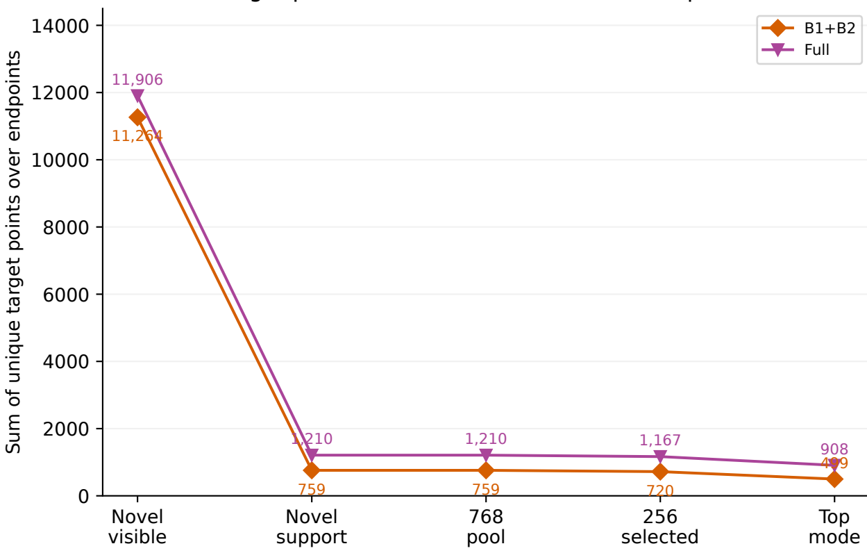
C. Target points across the evidence chain (epoch 60)
