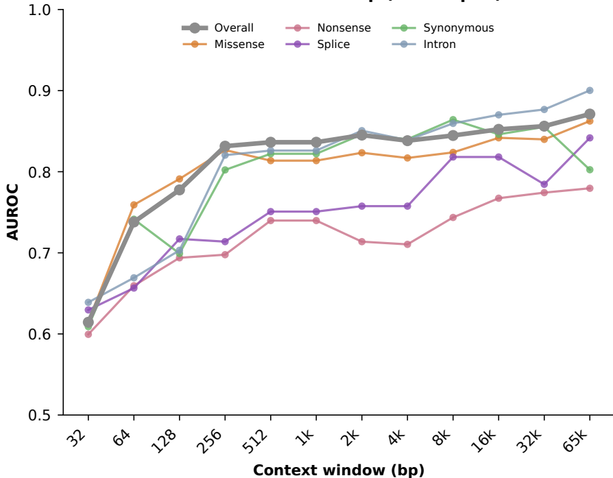
A. Context size sweep (unclamped)
