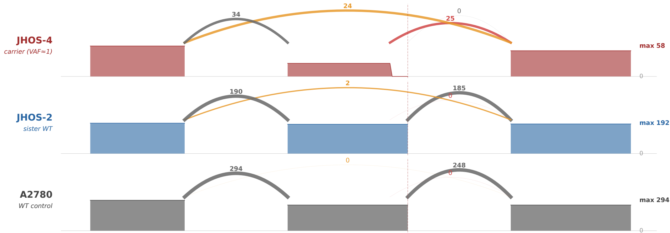
BRCA1 splice diagram (chr17:43,049,121-43,057,134 hg38, introns compressed)
