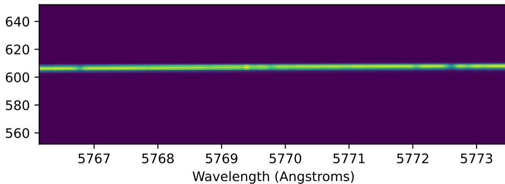
HARPS.2018-02-01T01:42:30.839.fits
