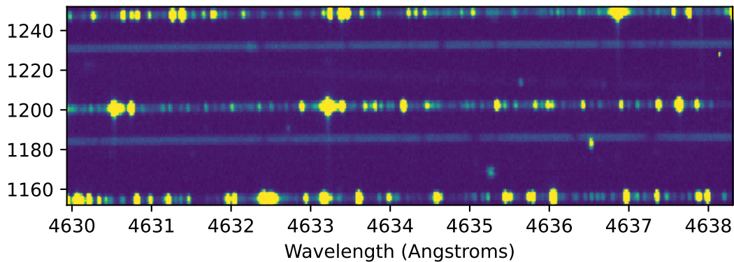
HARPS.2012-10-22T23:39:09.238.fits
