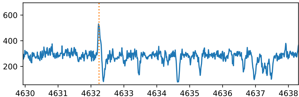
ADP.2014-09-26T16:52:17.823.fits
