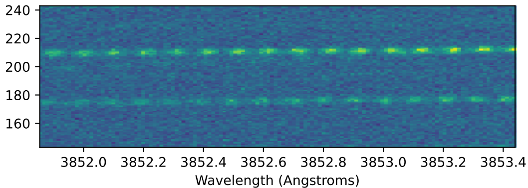
HARPS.2017-01-14T02:04:35.597.fits
