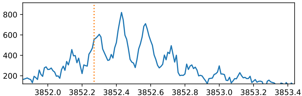
ADP.2017-01-15T01:03:41.689.fits
