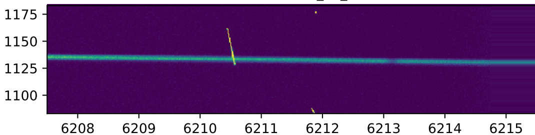
HARPS.2014-10-27T07_30_58.251.fits
