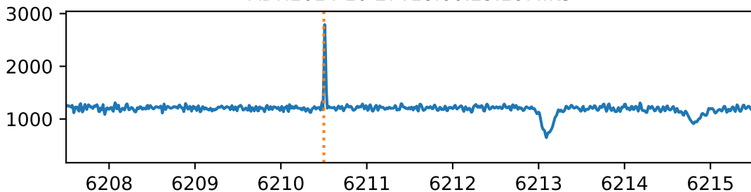
HARPS.2014-10-27T07_30_58.251.fits
