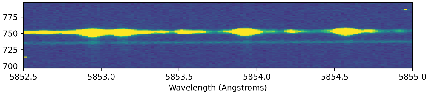
HARPS.2013-04-30T09_50_45.212.fits
