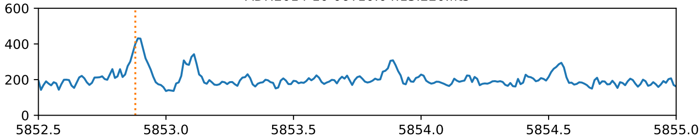
HARPS.2013-04-30T09_50_45.212.fits
