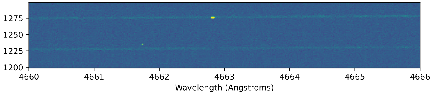
HARPS.2018-04-10T03_25_08.275.fits
