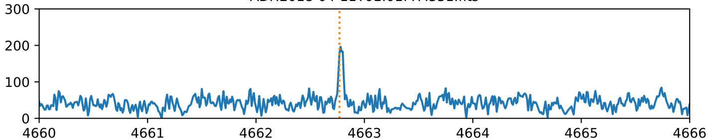
HARPS.2018-04-10T03_25_08.275.fits
