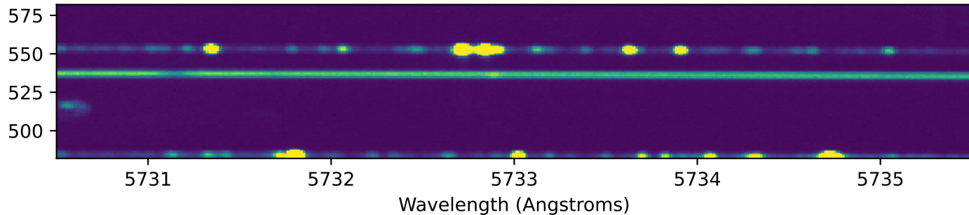
HARPS.2013-06-01T04_16_19.375.fits
