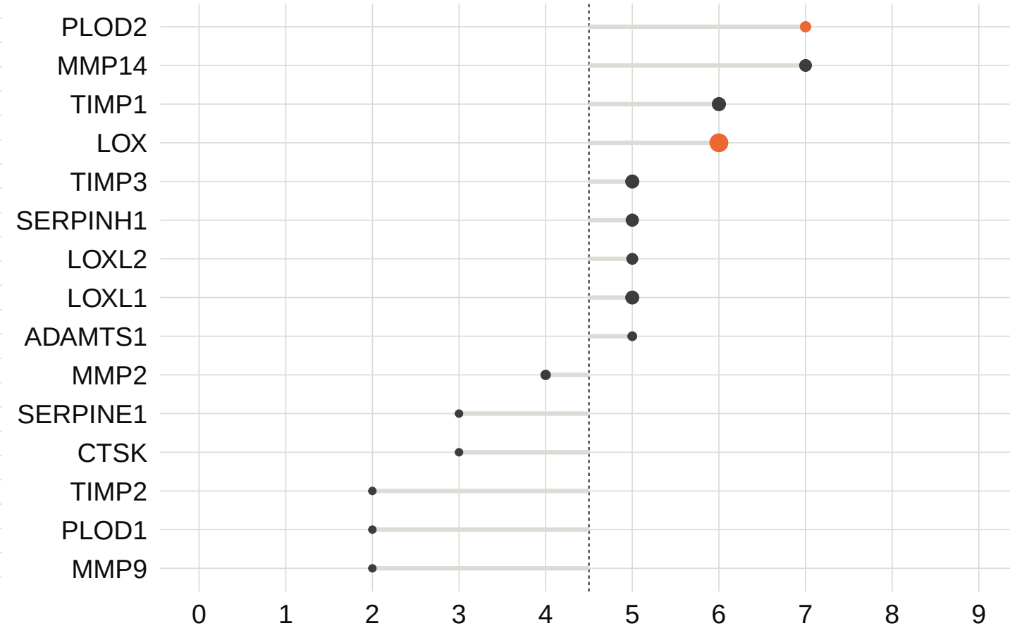
ecm_remodeling
