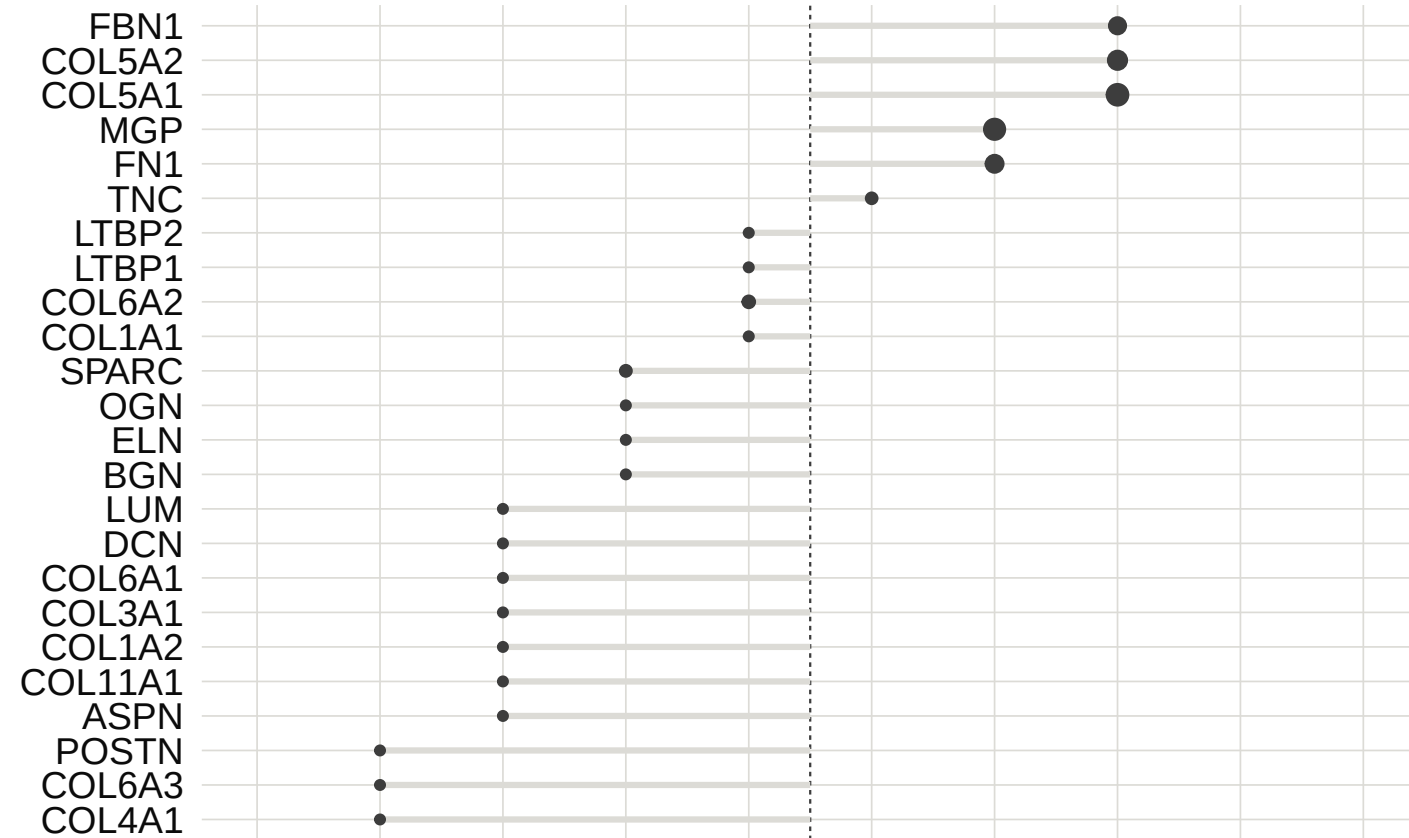
megakaryocyte_fibrosis_axis
