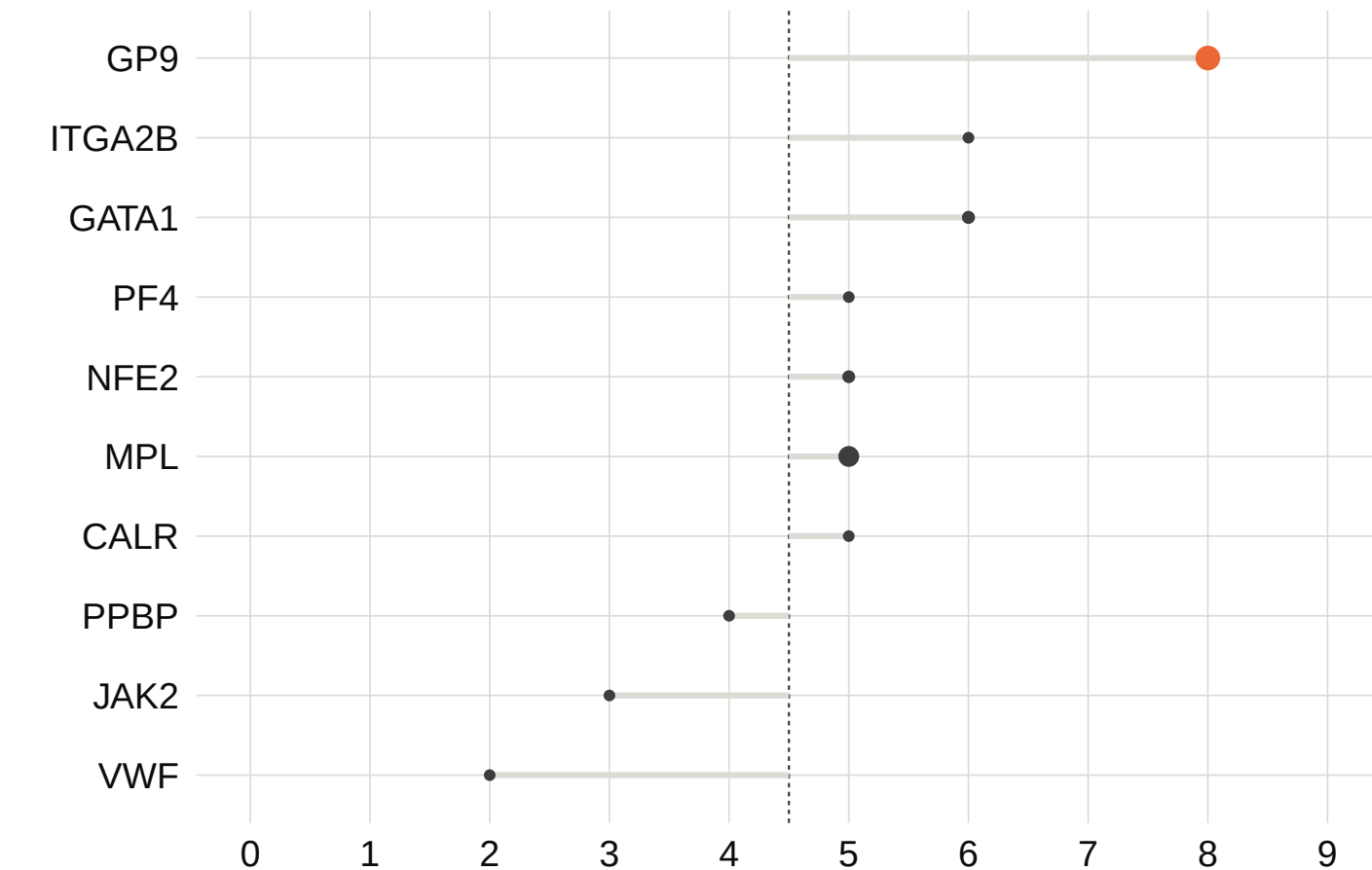
megakaryocyte_fibrosis_axis
