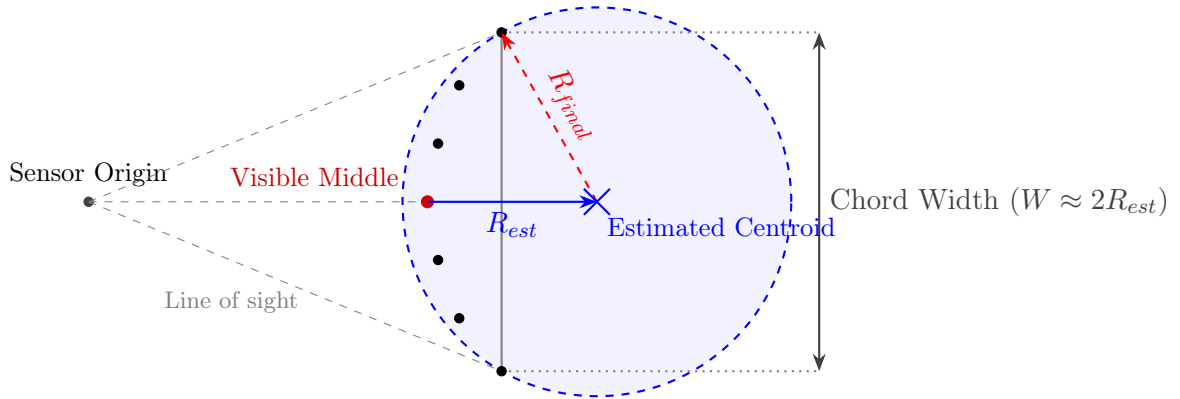
FIGURE 4.2: Custom spatial heuristic for circular primitive extraction.
