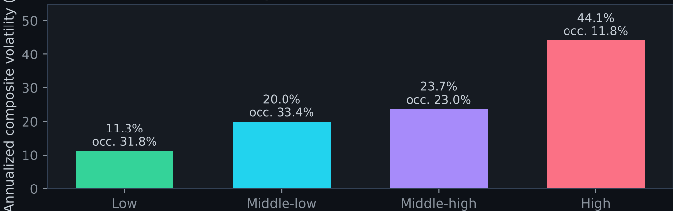
Four volatility-ordered DYNAMAX HMM states
