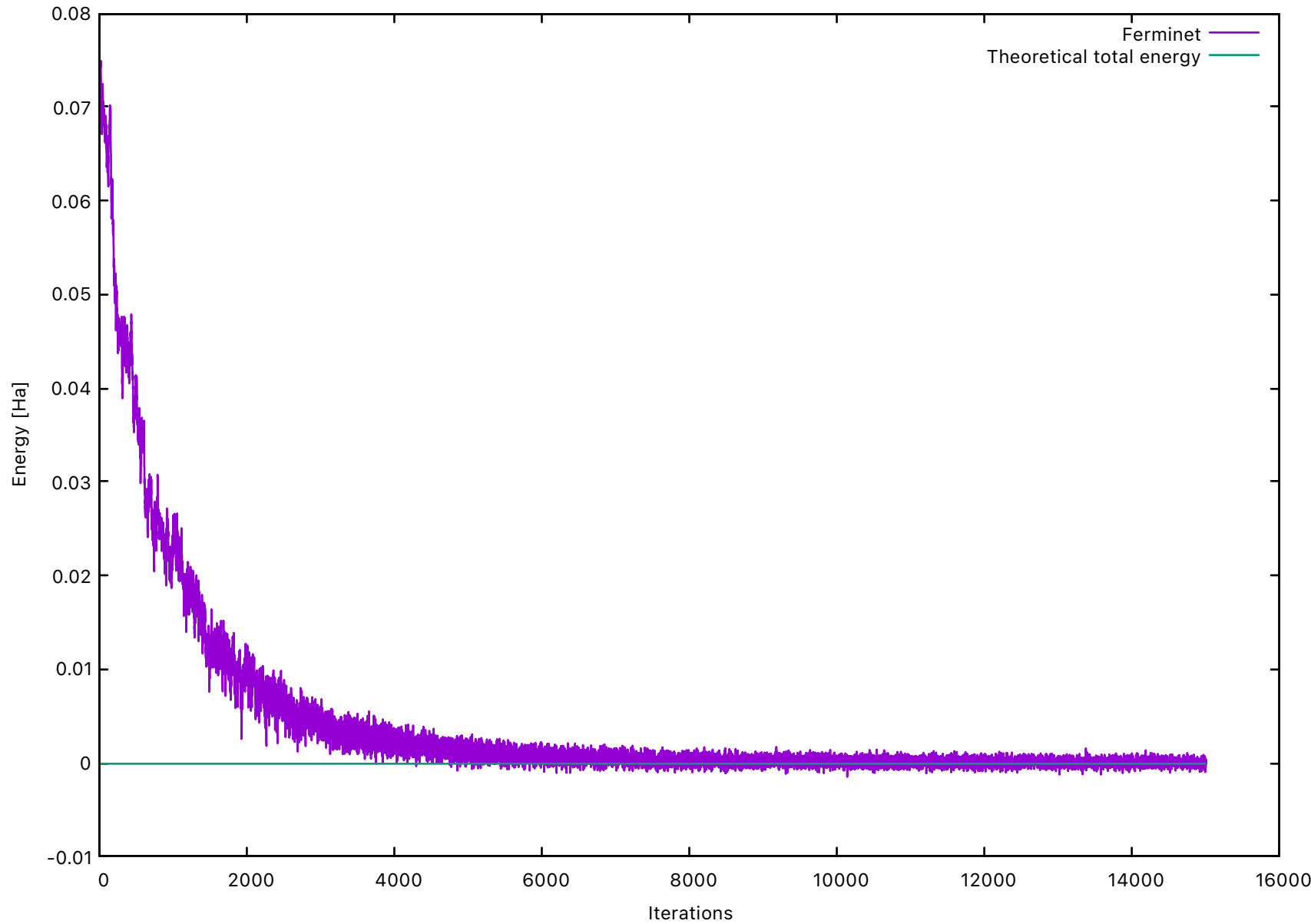
1D ideal gas, nspins = (1, 0)
