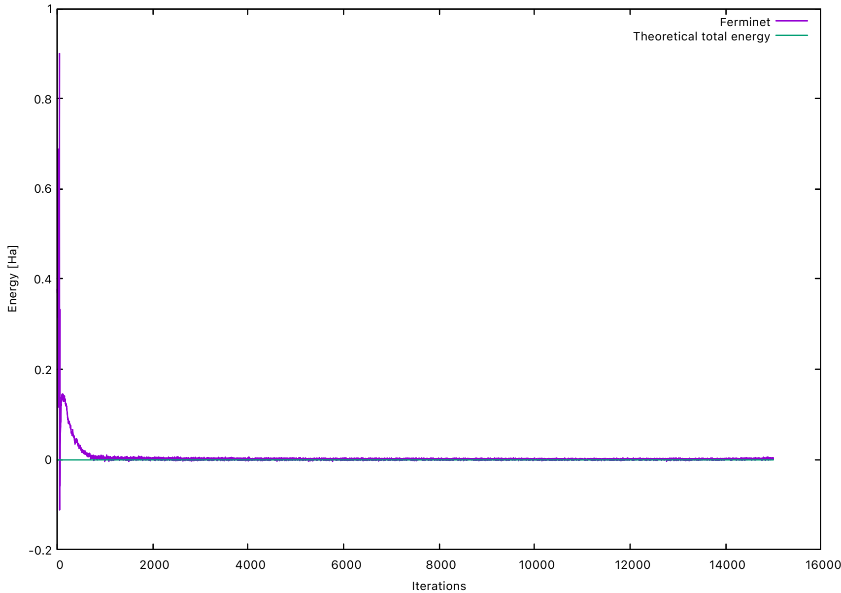
1D ideal gas, nspins = (1, 1)
