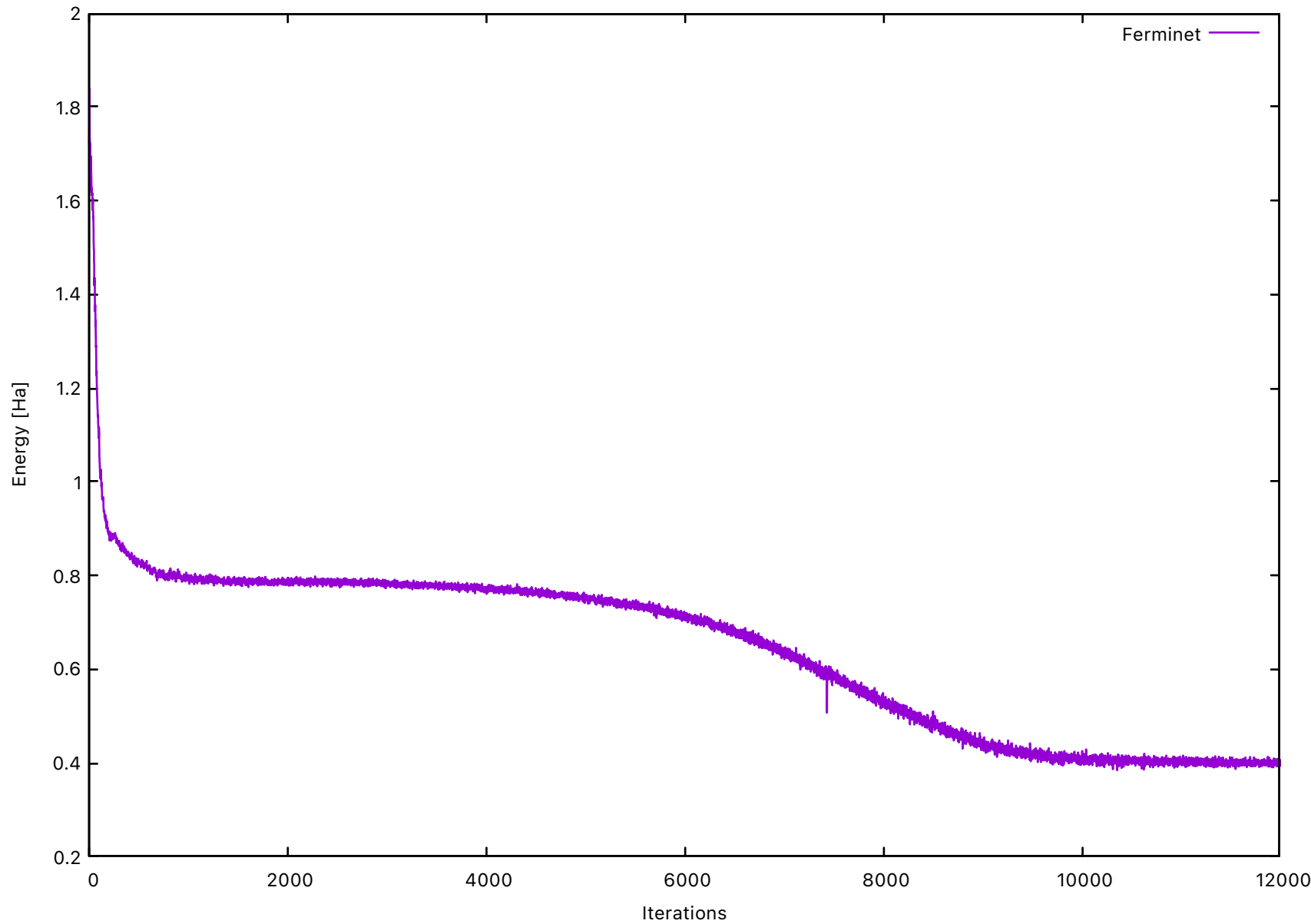
1D ideal gas, nspins = (2, 1)
