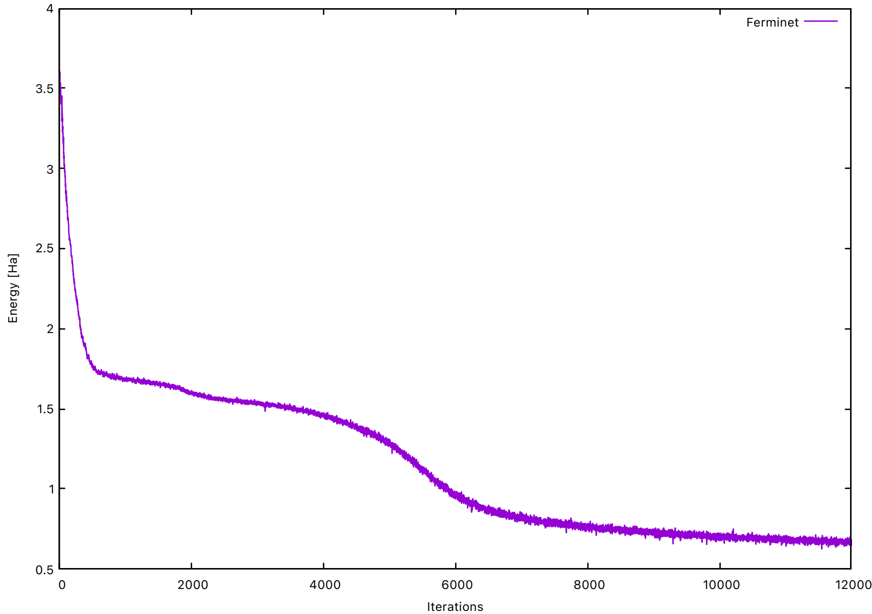
1D ideal gas, nspins = (2, 2)
