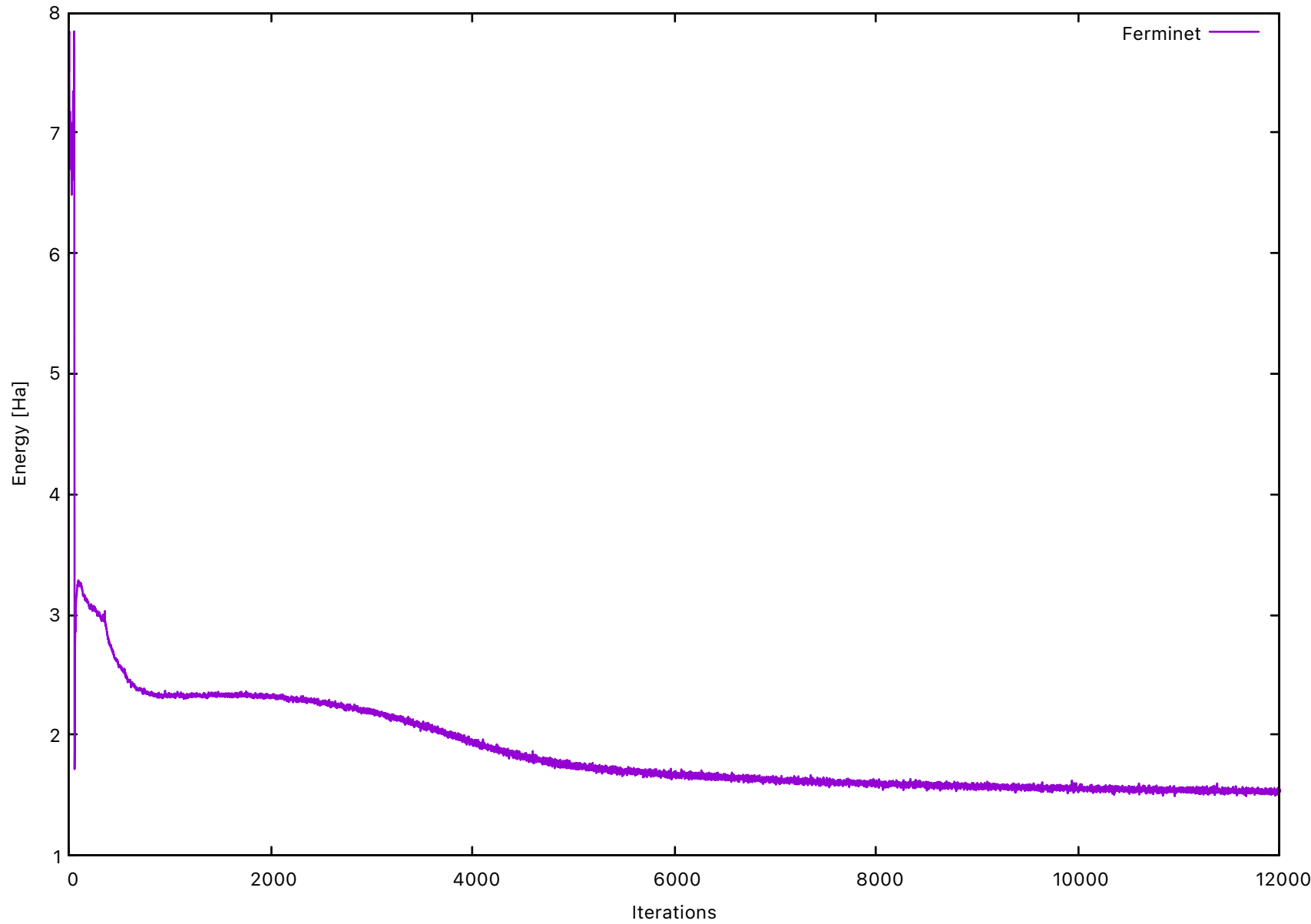
1D ideal gas, nspins = (3, 2)
