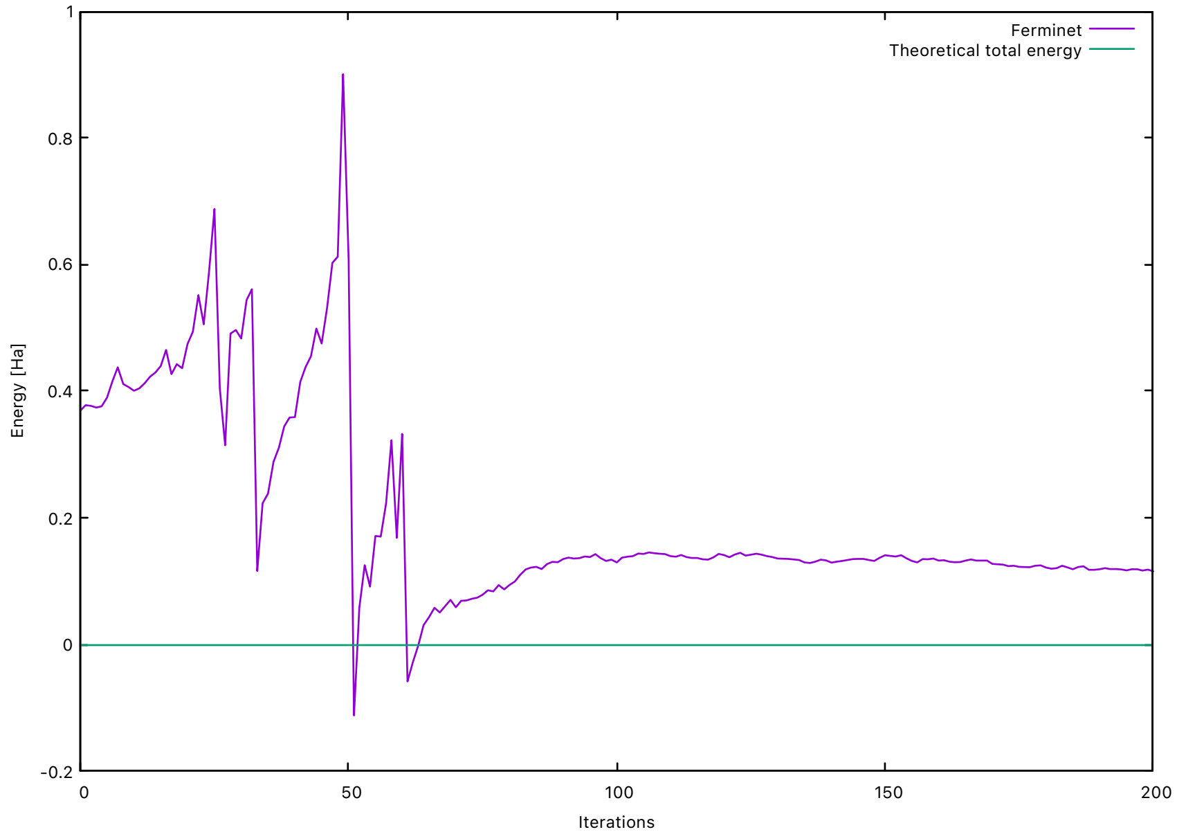
1D ideal gas, nspins = (1, 1), beginning of training
